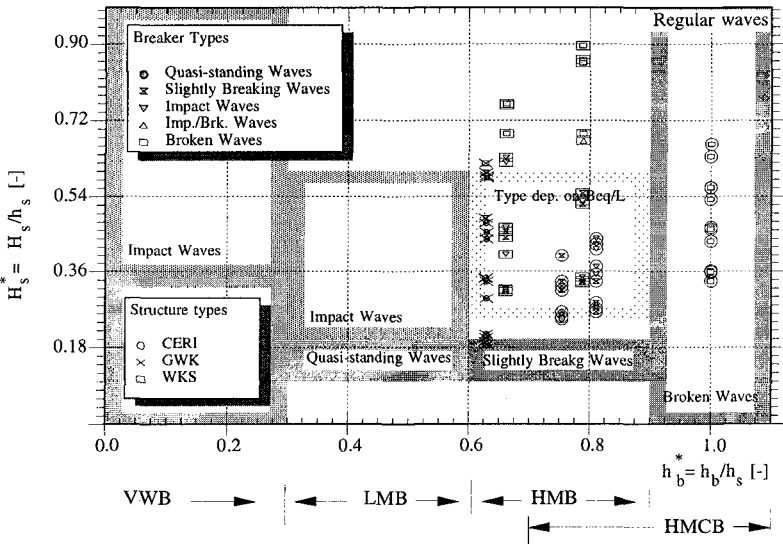
Figure 9. H_s^* vs h_b^* for Regular Wave Tests (All Data Sets)
