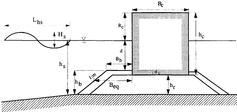
Figure 2. Definitions of Parameters
