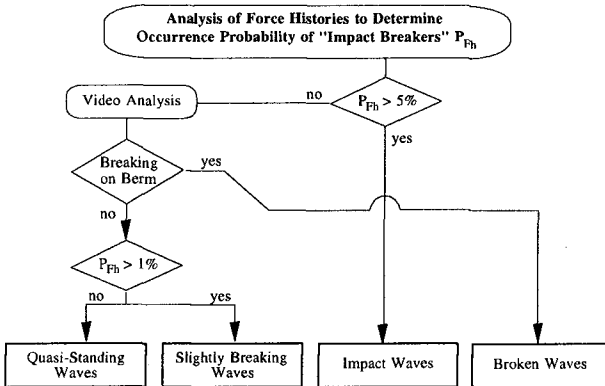
Figure 7. Flow Chart for Identification of Breaker Types for Random Wave Tests
