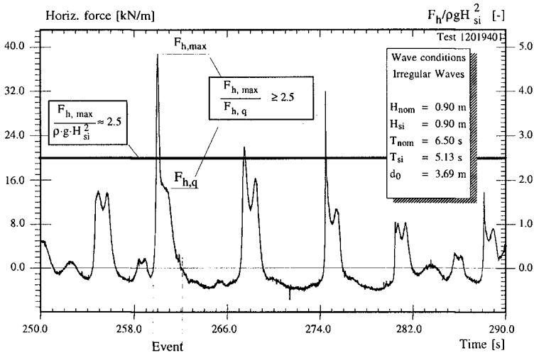
Figure 8. Definition of Impact Breakers from Force Time Series
