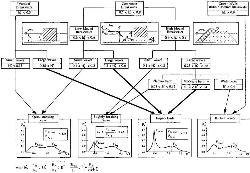
Figure 1. Parameter Map of PROVERBS ( Oumeraci, 1997 )
