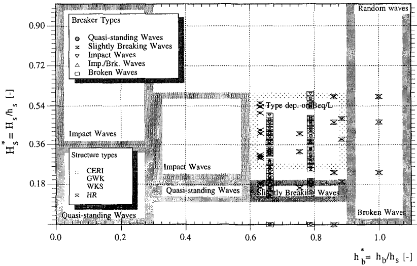
Figure 10. H_s^* vs h_b^* for Random Wave Tests (All Data Sets)
