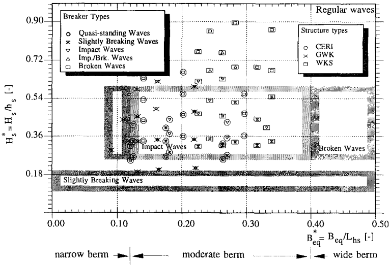
Figure 11. H_s^* vs B_{eq}^* for Regular Wave Tests ( h_b^* = 0.6 \div 0.9 , All Data Sets)
