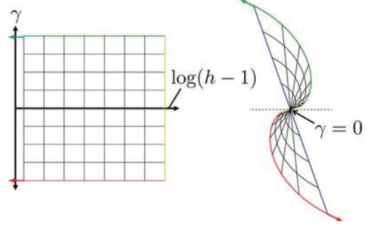
FIG. 6. (Color online) Mapping of the curved space in the h - \gamma plane to a flat plane in polar coordinates. A grid covering a subset of the h - \gamma plane (left) is shown mapped to a subset of the flat plane (right) by a coordinate change to r and \varphi as described in the text. The mapping is specifically shown for the leading-order asymptotics of the metric of the XY model given by Eqs. (64), for h ranging from 1.0009 to 2.0 and \gamma from -0.1 to 0.1 . The red and green arrows indicate that both \varphi and r diverge in the limit h \rightarrow 1^+ . Since g_{hh} = 0 for \gamma = 0 , the entire line \gamma = 0 maps to a single point, which is a singularity of the model.
