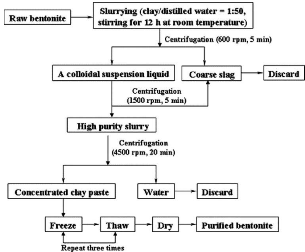
Scheme 2 Pretreatment process of raw bentonite (Wang et al. 2014)
