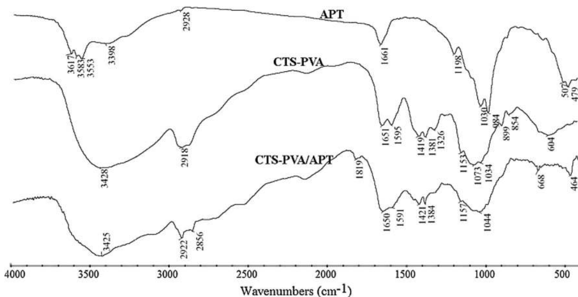
Fig. 18 FTIR spectra of chitosan-poly(vinyl alcohol)/attapulgit (CTS-PVA/APT) nanocomposite, chitosan-poly(vinyl alcohol) (CTS-PVA) and attapulgite (APT), the changes of peak confirm that the
