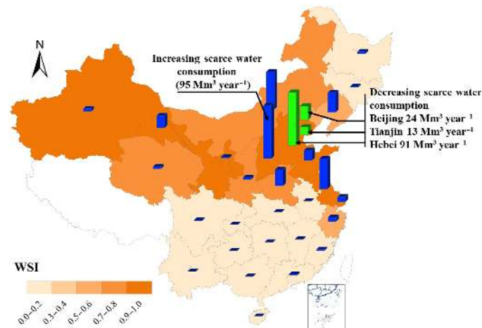
Fig. 5. Scarce water consumption changes triggered by the JJJ clean air policy. Green bars show the decrease in scarce water consumption in JJJ, and blue bars show the increase in scarce water consumption in other regions, with regions shaded according to the water stress index (WSI).
