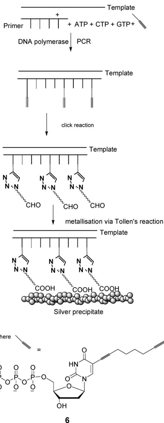
Fig. 7 Directed DNA metallization via click chemistry to create nano- and microscale assemblies.
