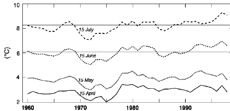
Fig. 5. Time-series of seasonal changes in sea surface temperatures (SST) in the south middle shelf stratum based on the GISST data set produced by the United Kingdom Meteorological Office (UKMO) (Parker et al., 1993). Note the trend toward increasing SST in the 15 June and 15 July time series.
