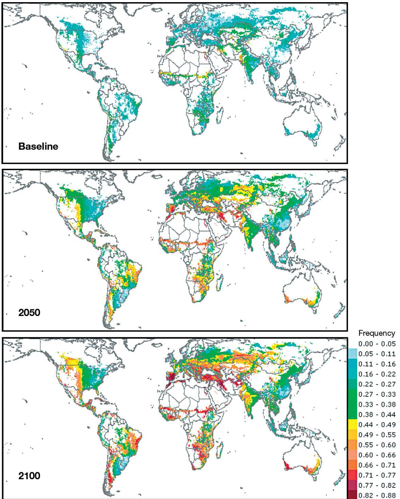
Fig. 3. Global drought disaster frequencies for the cropland growing season (3 mo Palmer Drought Severity Index < -3 , in growing season) for baseline (1949–2006), 2050 and 2100 projections
