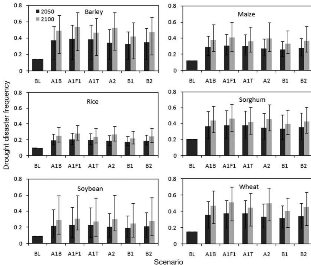
Fig. 5. Change in global drought disaster frequencies (3 mo Palmer Drought Severity Index <-3, in growing season) of major crop sown areas for 20 general circulation model (GCM) patterns and 6 SRES emissions scenarios (A1B, A1F1, A1T, A2, B1 and B2). BL: baseline. Data are average of 20 GCMs; error bars: the range of individual GCM results
