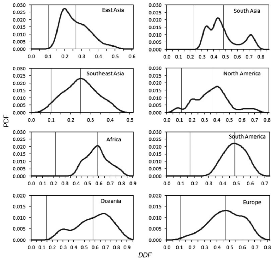
Fig. 6. Probability density function (PDF) distribution of the drought disaster frequency ( DDF ) for the different regions, predicted by 20 general circulation models and 6 SRES emissions scenarios (120 predictions in total) for 2100. The left vertical line shows the average DDF of the baseline; the right vertical line shows the average DDF in 2100 under all scenarios
