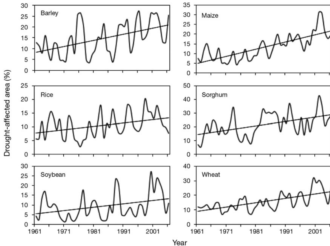
Fig. 1. Percentage of drought disaster-affected area of the major crop sown regions from 1961 to 2006. Straight lines: linear trend
