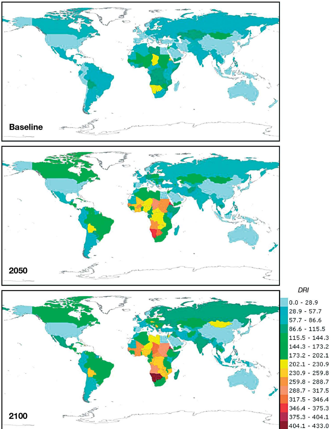
Fig. 7. Global country-specific drought risk index ( DRI ) of cropland for baseline (1961–2006), 2050 and 2100 projections
