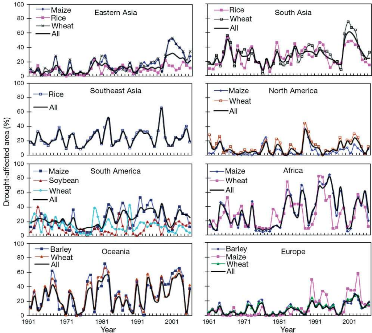
Fig. 2. Percentage of drought disaster-affected area of major cropland areas (3 mo Palmer Drought Severity Index < -3 , in growing season) in different regions
