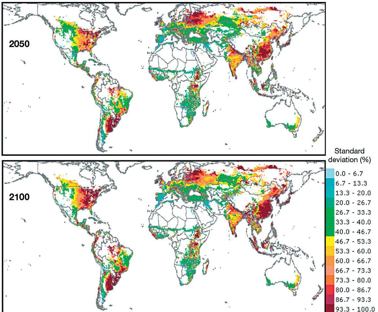
Fig. 4. Relative standard deviation (%) of drought disaster frequency change of general circulation model patterns and scenarios
