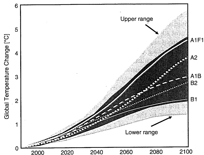
Figure 1. Global warming futures according to various greenhouse-gas emission scenarios developed by the Intergovernmental Panel on Climate Change (Source: IPCC, 2007).
