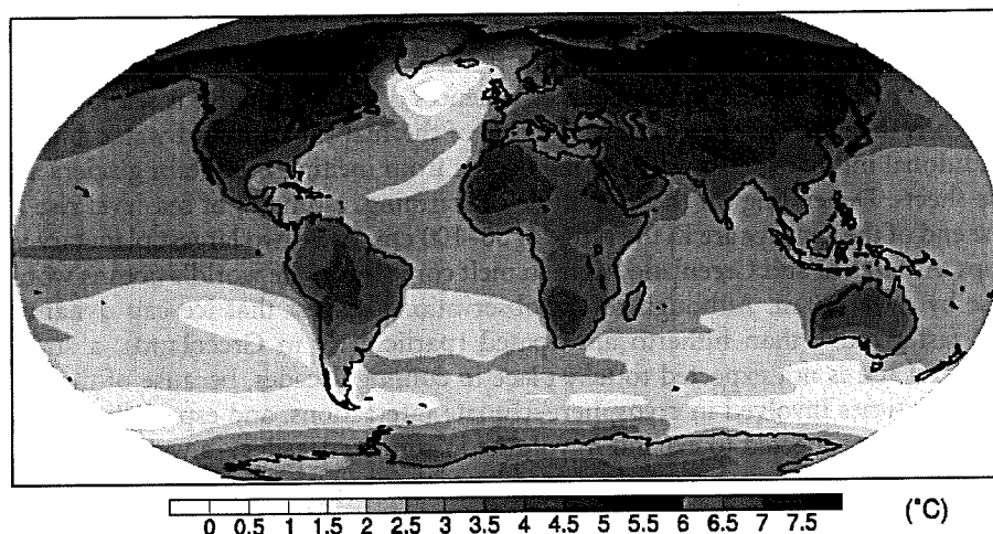
Figure 2. Changes in temperature between current (1980–1999) and future (2080–2099) climates based on ensemble model simulations (Source: IPCC, 2007).
