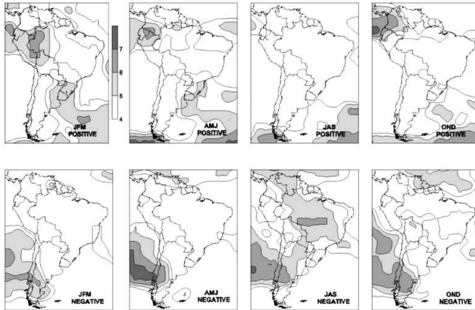
Figure 3. Number of models depicting (top) positive changes and (bottom) negative changes in maps of Figure 2.
