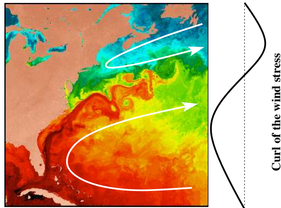
FIGURE 3. A satellite image of the sea surface temperature (SST) over the north-western North Atlantic (U.S. National Oceanic and Atmospheric Administration), together with a sketch of the associated double-gyre circulation. An idealized view of the amount of potential vorticity injected into the ocean circulation by the trade winds, westerlies and polar easterlies is shown to the right.
