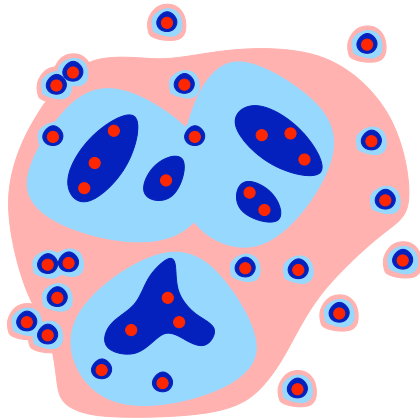
FIGURE 6. A conjectural view of stochastic classification for GCMs, using the concept of random attractors. Each point in red represents a GCM in which stochastic parametrizations are switched off, while each gray area represents a cluster of stochastically equivalent GCMs for a given level of the noise.
