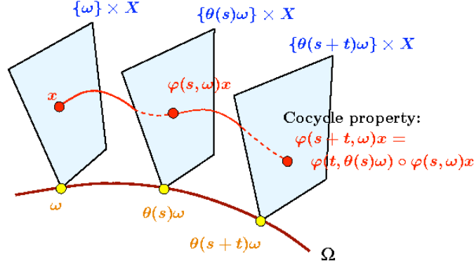
FIGURE 10. Random dynamical systems (RDS) viewed as a flow on the bundle X \times \Omega = \text{“dynamical space”} \times \text{“probability space.”} For a given state x and realization \omega , the RDS \varphi is such that \Theta(t)(x, \omega) = (\theta(t)\omega, \varphi(t, \omega)x) is a flow on the bundle.
