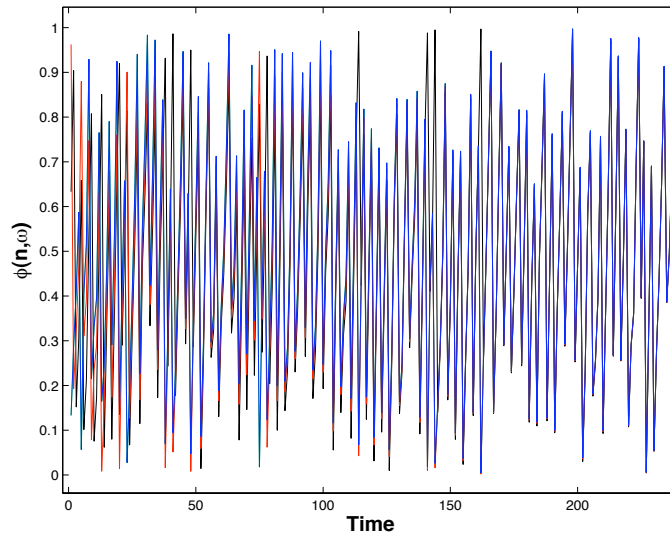
FIGURE 9. Synchronization by additive noise: three distinct trajectories (in blue, red and black) of x_{n+1} = F_{\tau, \epsilon; \omega}(x_n) , with F_{\tau, \epsilon; \omega} given by (B.1); the three trajectories start from three initial points on the circle, but are driven by the same realization \omega of the noise, and thus converge to the same random fixed point a(\omega) , which is moving with time. The parameters are \epsilon = 0.5 , \tau = 0.283 and \sigma = 0.3 , and the corresponding Lyapunov exponent is \lambda \simeq -0.0104 .
