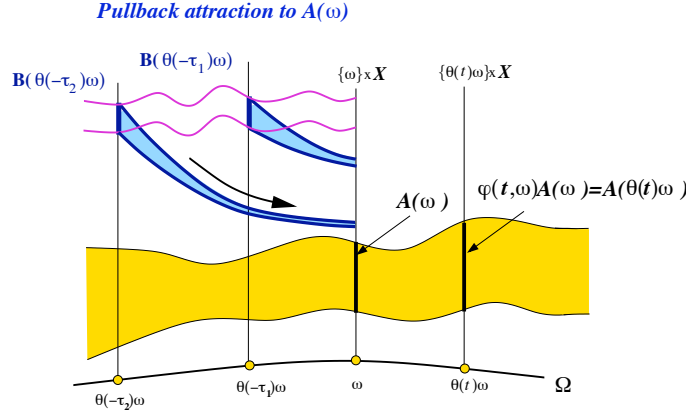
FIGURE 11. Schematic diagram of a random attractor \mathcal{A}(\omega) , where \omega \in \Omega is a fixed realization of the noise. To be attracting, for every set B of X in a family \mathfrak{B} of such sets, one must have \lim_{t \rightarrow +\infty} \text{dist}(B(\theta(-t)\omega), \mathcal{A}(\omega)) = 0 with B(\theta(-t)\omega) := \varphi(t, \theta(-t)\omega)B ; to be invariant, one must have \varphi(t, \omega)\mathcal{A}(\omega) = \mathcal{A}(\theta(t)\omega) . This definition depends strongly on \mathfrak{B} ; see [112] for more details.
