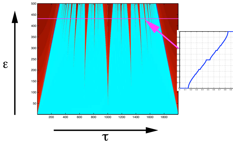
FIGURE 7. Arnol’d tongues for the family of diffeomorphisms of the circle; units for \tau and \epsilon are 5 \cdot 10^{-4} and 10^{-4} respectively. Devil’s staircase in the cross-section to the right.
