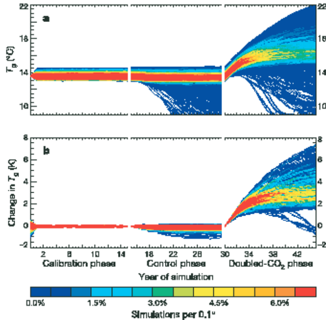
FIGURE 1. Frequency distributions of global mean, annual mean, near-surface temperature ( T_g ) for (a) 2,017 GCM simulations, and doubled \text{CO}_2 ; and for (b) a subset of 414 stable simulations, without substantial climate drift (from [8]).
