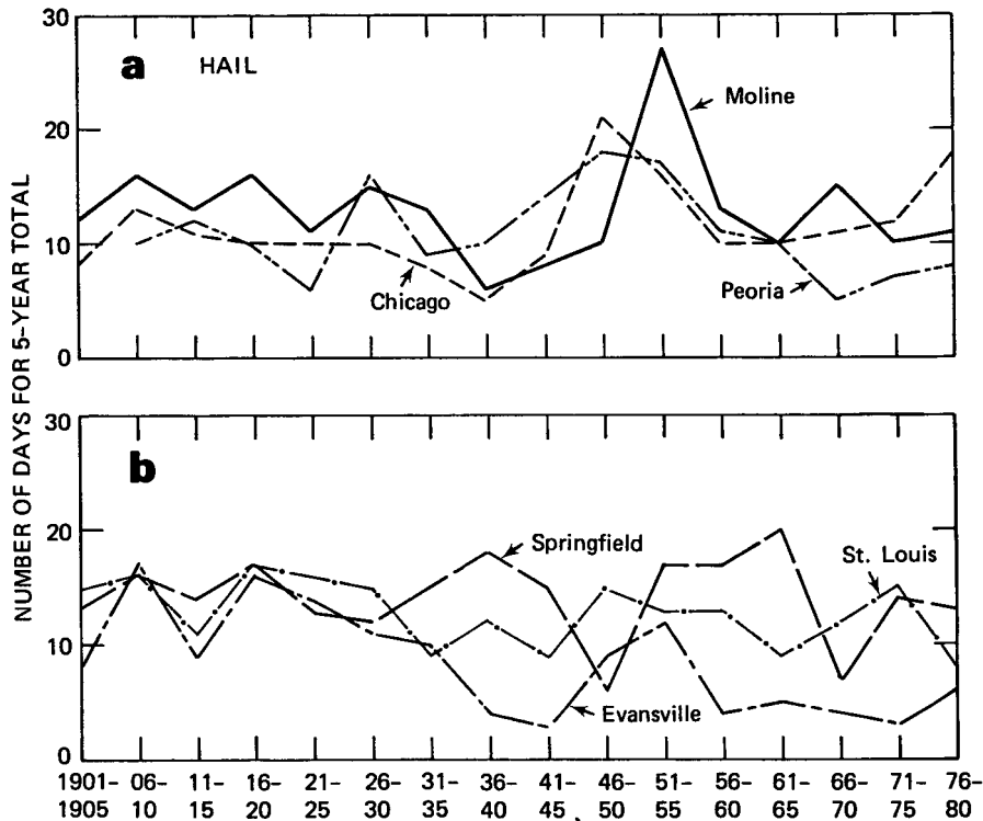
Figure 19. Number of days with hail (5-year totals)
