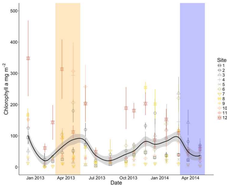
Figure 4. Mean ( n = 6 ) benthic chlorophyll a ( mg\ m^{-2} ) for each ecosystem metabolism study site for each date sampled. Vertical lines are \pm 1 standard error. The black line and gray bands represent the average and standard error of all estimates of chlorophyll a across all sites per date. The orange and blue bands highlight the spring snowmelt window following high-snow winter (HS, 2012/2013) and low-snow winter (LS, 2013/2014), respectively.
