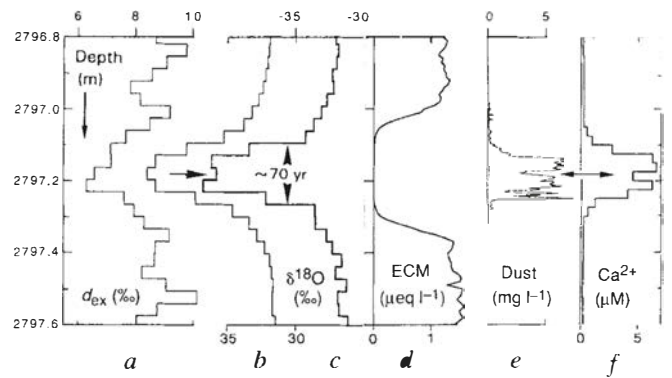
FIG. 4 Profiles of five parameters through 'event 1', a rapid climatic oscillation ( \sim 70 yr duration) at the culmination of the Eemian interglacial, \sim 115 kyr BP. a, Deuterium excess 15 ; b, oxygen isotope ratio 7 ; c, same as b, but deconvoluted to account for diffusion (estimated diffusion length 3 cm); d, acidity measured by ECM in microequivalents per litre 31 ; e, dust concentration measured from scattered laser light and calibrated by Coulter Counter by integrating size distribution 33 ; f, calcium ion concentration 38 .
