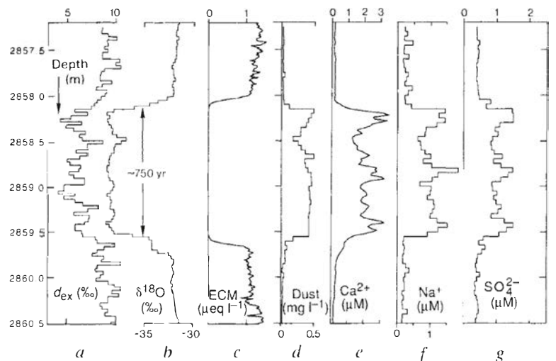
FIG. 5 Profiles of oxygen isotope ratio 7 , calcium ion concentration 38 , acidity by ECM 31 , dust 33 , deuterium excess 15 , sodium and sulphate 41 through 'event 2', a climate oscillation sustained for \sim 750 yr in the initial stages of the Eemian interglacial \sim 131 kyr BP.
