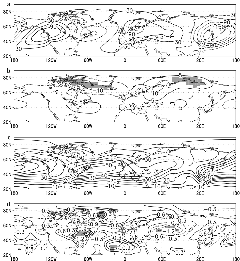
Fig. 12 Transient and mean atmospheric circulation in middle and high boreal latitudes in 4\times\text{CO}_2 ct and modifications introduced the interactive ice sheets: winter (DJF) geopotential height anomalies relative to the zonal mean at 500 hPa a from 4\times\text{CO}_2 ct and b 4\times\text{CO}_2 minus 4\times\text{CO}_2 ct; storm-track in c 4\times\text{CO}_2 ct and d 4\times\text{CO}_2 minus 4\times\text{CO}_2 ct. Units are geopotential meters (gpm). Contour lines are plotted every 30, 3, 5 and 0.3 gpm in (a), (b), (c), and (d), respectively. The storm track is defined as the band-pass filtered standard deviation of the geopotential height field at 500 hPa, as in Blackmon (1976). The grey shading indicates areas where the statistical significance exceeds the 95% confidence level
