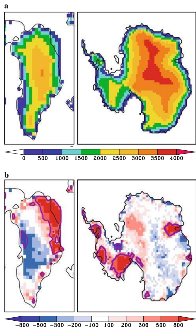
Fig. 2 a Topography of CTRL ice sheets and b anomalies with ETOPO5 (m) in the ice sheet model grid. The purple contour line indicates anomalies exceeding 500 m in magnitude. The black contour line indicates the zero iseline of CTRL topography in the ice sheet model
