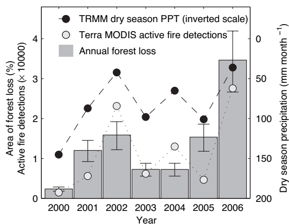
Fig. 4. Interannual rate of forest loss in southern Borneo (south of 1^{\circ}\text{S} ) shown as percentage of area with >50\% woody cover in 2000 (33), average dry season precipitation based on TRMM precipitation (14), and Terra-MODIS active fire detections (20). Error bars on forest loss rates indicate the omission errors (positive) and commission errors (negative).
