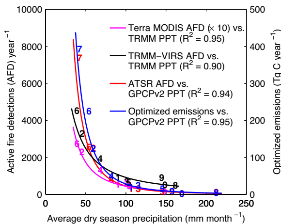
Fig. 3. Relation between average precipitation rates during peak fire season and satellite-derived active fire detections (AFD). Optimized emissions for southern Borneo (south of 1^{\circ}\text{S} ), the region most impacted by ENSO-induced interannual variability in precipitation rates, are also shown. Because of variability in the timing of the dry season, here we defined average dry season precipitation as the mean monthly precipitation during the 3 consecutive months with lowest rainfall. The numbers in the graph denote the year (7 = 1997, 0 = 2000, 1 = 2001, etc., through 6 = 2006); correlation coefficients are based on a power fit. Data sources include TRMM (14) and Global Precipitation Climatology Project version 2 (GPCV2) (36) for precipitation and TRMM-Visible Infrared Scanner (VIRS) (37), (Advanced) Along Track Scanning Radiometer (A)ATSR (38), and Terra-MODIS (20) for active fire detections. Differences in precipitation rates between GPCV2 ( 2.5^{\circ} \times 2.5^{\circ} ) and TRMM ( 0.25^{\circ} \times 0.25^{\circ} ) are caused, in part, by differences in spatial resolution. The large fires in early 1998 in eastern Borneo burned outside this study region.
