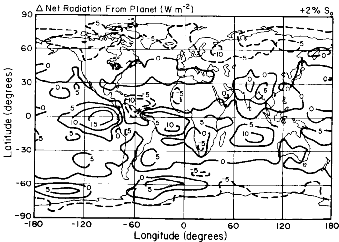
Fig. 7. Annual mean radiation changes in the climate model for two percent increase of S_0 (left) and doubled CO_2 (right). In Figs. 7, 8, 10 and 11 "percent" change refers to the full range of the quantity, e.g., a change from 60 percent albedo to 50 percent albedo is defined to be a 10 percent change.
