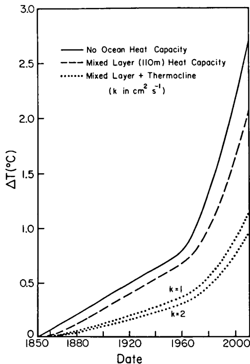
Fig. 18. Global mean warming computed for the CO 2 and trace gas scenarios in Table 4.
