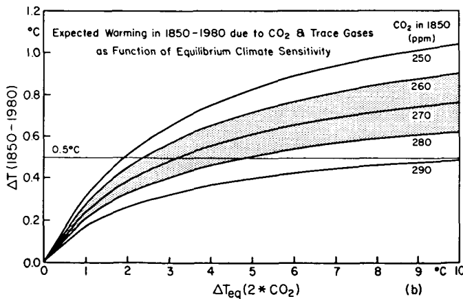
Fig. 17. Computed global warming between 1850 and 1980 as a function of the equilibrium climate sensitivity for doubled CO 2 (315 ppm → 630 ppm), ΔT eq (2*CO 2 ). Results are shown for five values of the assumed abundance of CO 2 in 1850; the shaded area covers the range 270±10 ppm recommended by WMO (1983). (a) includes only CO 2 growth, while (b) also includes the trace gas growths of Table 4. In all cases CO 2 increases linearly from the 1850 abundance to 315 ppm in 1958 and then according to measurements of Keeling et al. (1982).
