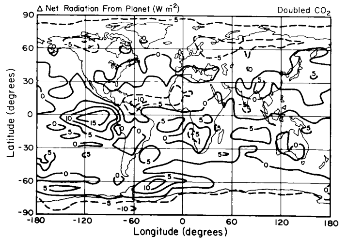
Fig. 7. Annual mean radiation changes in the climate model for two percent increase of S_0 (left) and doubled CO_2 (right). In Figs. 7, 8, 10 and 11 "percent" change refers to the full range of the quantity, e.g., a change from 60 percent albedo to 50 percent albedo is defined to be a 10 percent change.
