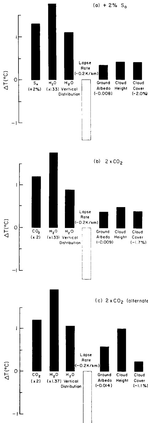
Fig. 6. Contributions to the global mean temperature rise in the S_0 and CO_2 experiments as estimated by inserting changes obtained in the 3-D experiments into 1-D radiative convective model. (a) +2 percent S_0 experiment, (b) doubled CO_2 experiment, and (c) doubled CO_2 experiment for alternate control run with greater sea ice.
