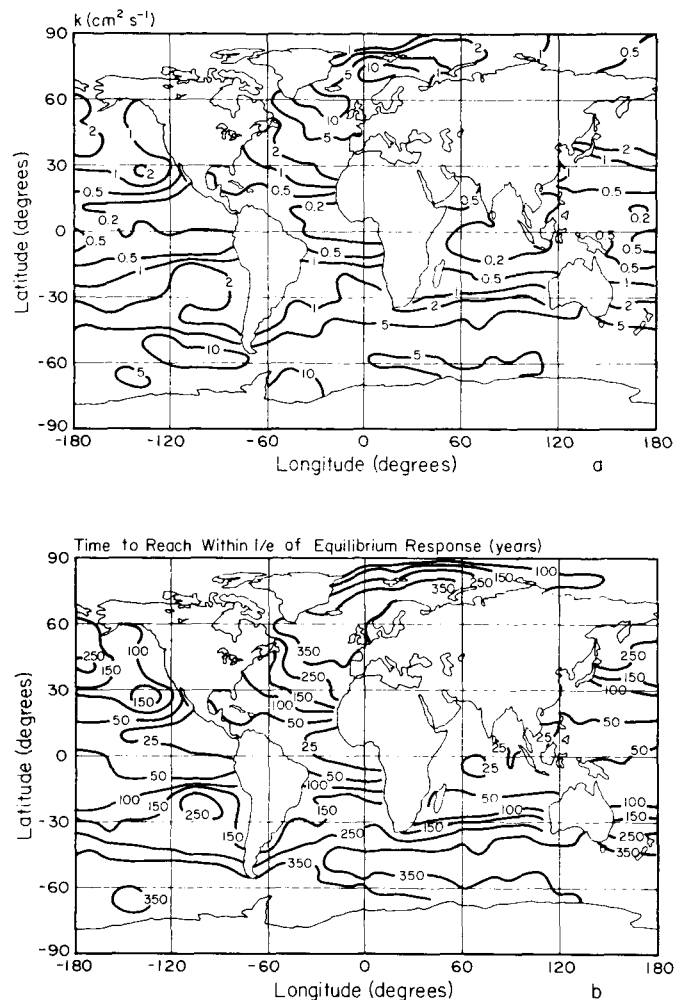
Fig. 15. (a) Geographic distribution of effective thermocline diffusion coefficient, k ( \text{cm}^2\text{s}^{-1} ). k is derived from Eq. 25 and the global distribution of N^2 , the latter obtained from the ocean data of Levitus (1982). (b) Geographic distribution of the 63 percent response time for surface temperature response to doubled \text{CO}_2 in the atmosphere. Only geographic variability of k and mixed layer depth are accounted for. \Delta T_{\text{eq}}(2*\text{CO}_2) is taken as 4.2^\circ\text{C} everywhere. The flux into the ocean is from Eq. (24).
