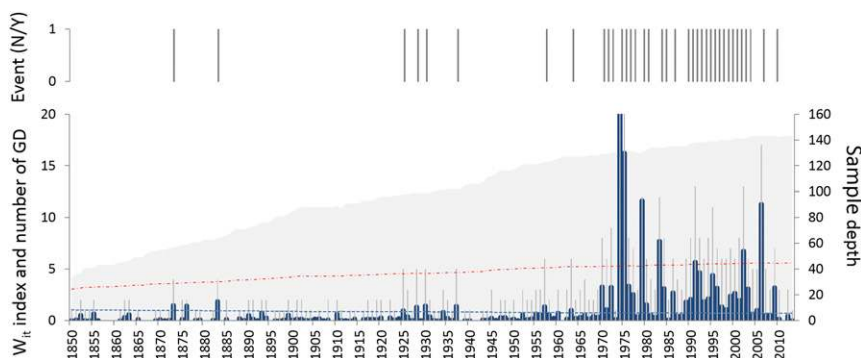
Fig. 3. Snow avalanche reconstruction based on tree-ring records from 144 broadleaved and conifer trees. ( Upper ) Chronology of 38 reconstructed snow avalanches. N, no; Y, yes. ( Lower ) W_{it} index (blue columns), the number of GDs (gray columns) observed each year, the sample depth (i.e., number of trees available for analysis in any given year), and the related W_{it} and number of GD thresholds (blue and red lines, respectively) used to distinguish avalanche signal from noise.
