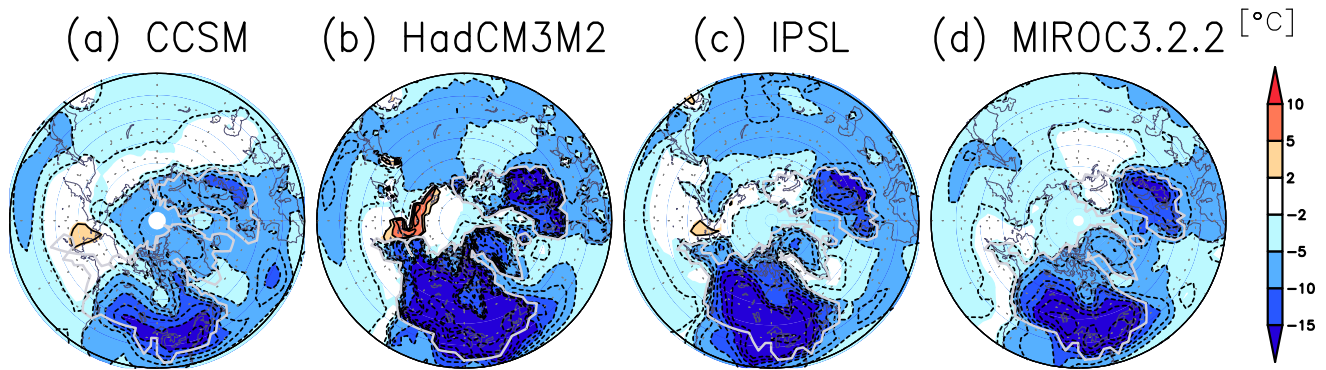
Fig. 4. Change in summer surface air temperature for a subset of PMIP2 simulations: (a) CCSM, (b) HadCM3M2, (c) IPSL, (d) MIROC3.2. The lapse rate effect is extracted by assuming the lapse rate= 5\text{ K km}^{-1} for each modelled ice sheet topography.
