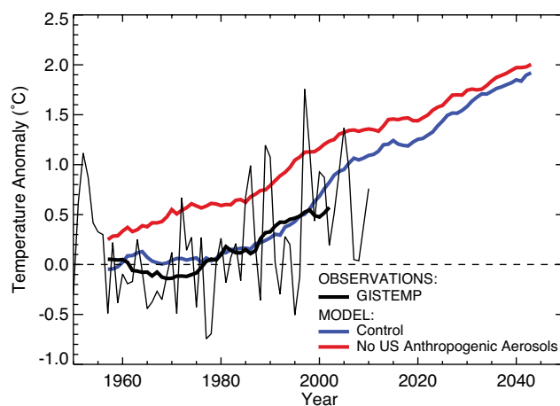
Fig. 9. 1950–2050 trends in annual mean surface air temperatures over the mid-Atlantic US (boxed region in Fig. 2). Observations (GISTEMP) are compared to the control simulation including greenhouse and aerosol forcings and to the sensitivity simulation with no US anthropogenic aerosols. Observations are the anomaly relative to the observed 1951–1980 mean and are shown for individual years (thin line) and for a 15-yr moving average (thick line). Model temperatures are the 5-member ensemble mean anomaly relative to the 1951–1980 mean of the control simulation, and are shown as 15-yr moving averages.
