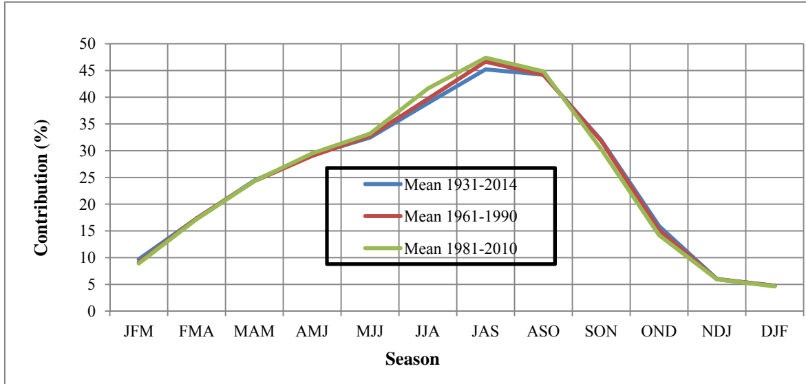
Fig. 5 Seasonal contributions to annual rainfall in N'zerekore.
