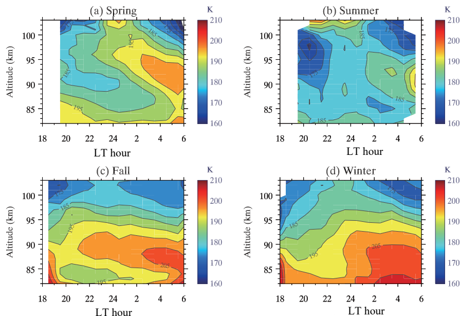
Figure 2. Lidar-observed nighttime hourly mean temperature composite in (a) spring, (b) summer, (c) fall and (d) winter.
