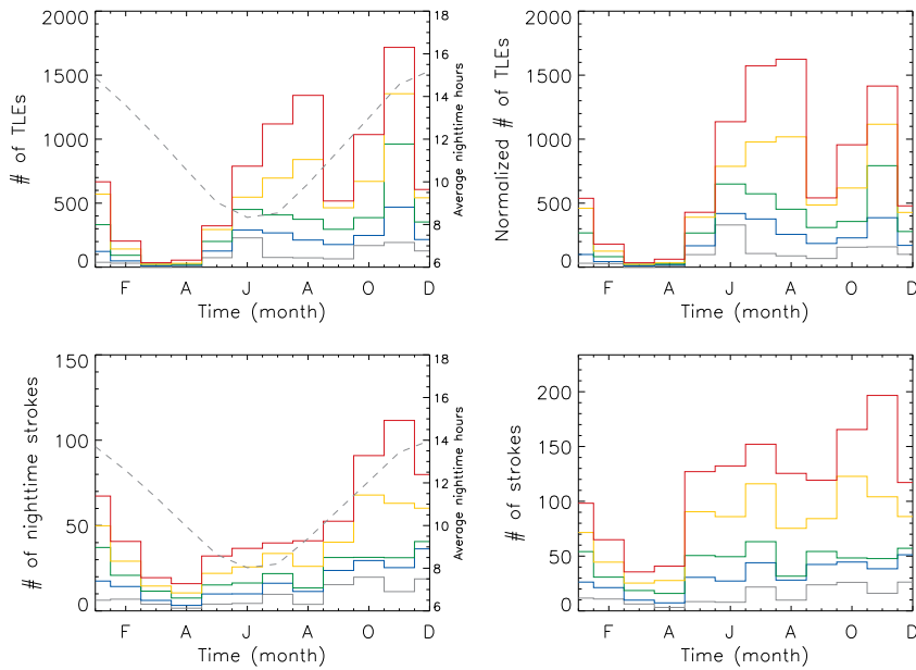
Figure 8. Cumulative number of observed TLEs (top) and WLLN CG strokes (bottom) per month including data from the start of the sample (January 2009) to the end of 2009, 2010, 2011, 2012 and 2013 (respectively in grey, blue, green, yellow and red). Panels in the left column show TLEs and nighttime strokes; the average seasonal cycle of nighttime hours is shown in dashed grey. Panels in the right column show TLEs normalized to a constant 12-hour nighttime and WLLN strokes during the whole day. WLLN data are scaled by a factor 10^4 and averages calculated over the rectangular shapes shown in Fig. 3.
