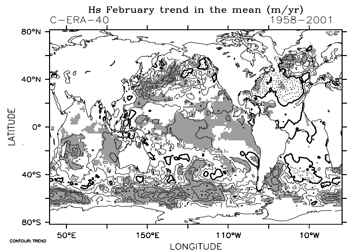
Figure 9. Trends in the February monthly mean H_s (C-ERA-40, upper) and the 99% quantiles (lower). Areas where the trend is significant at the 5% level are shaded. The significance is estimated using the non-parametric Mann-Kendall test as described in Wang, Swail (2001).
