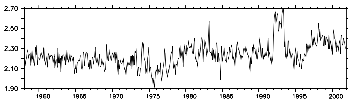
Figure 2. Timeseries of the monthly mean, globally averaged H_s from ERA-40. Monthly means are computed from the 6-hourly fields between 81^\circ\text{S} and 81^\circ\text{N} , and a latitudinal correction has been applied.
