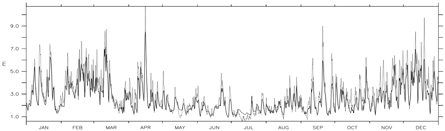
Figure 1. Measured (dotted) and modelled (solid) H_s at buoy 46001 ( 148.3^\circ\text{W} , 56.3^\circ\text{N} ) in 1988.
