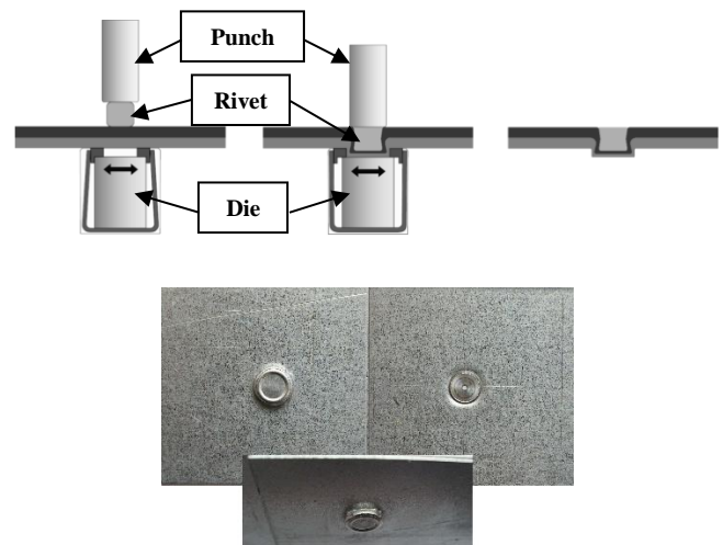
Fig. 1. Principle of ClinchRivet process
