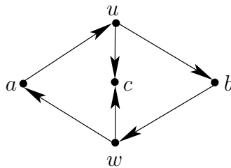
Figure 1: Candidate c is undominated, but cannot be made a winner by cloning
