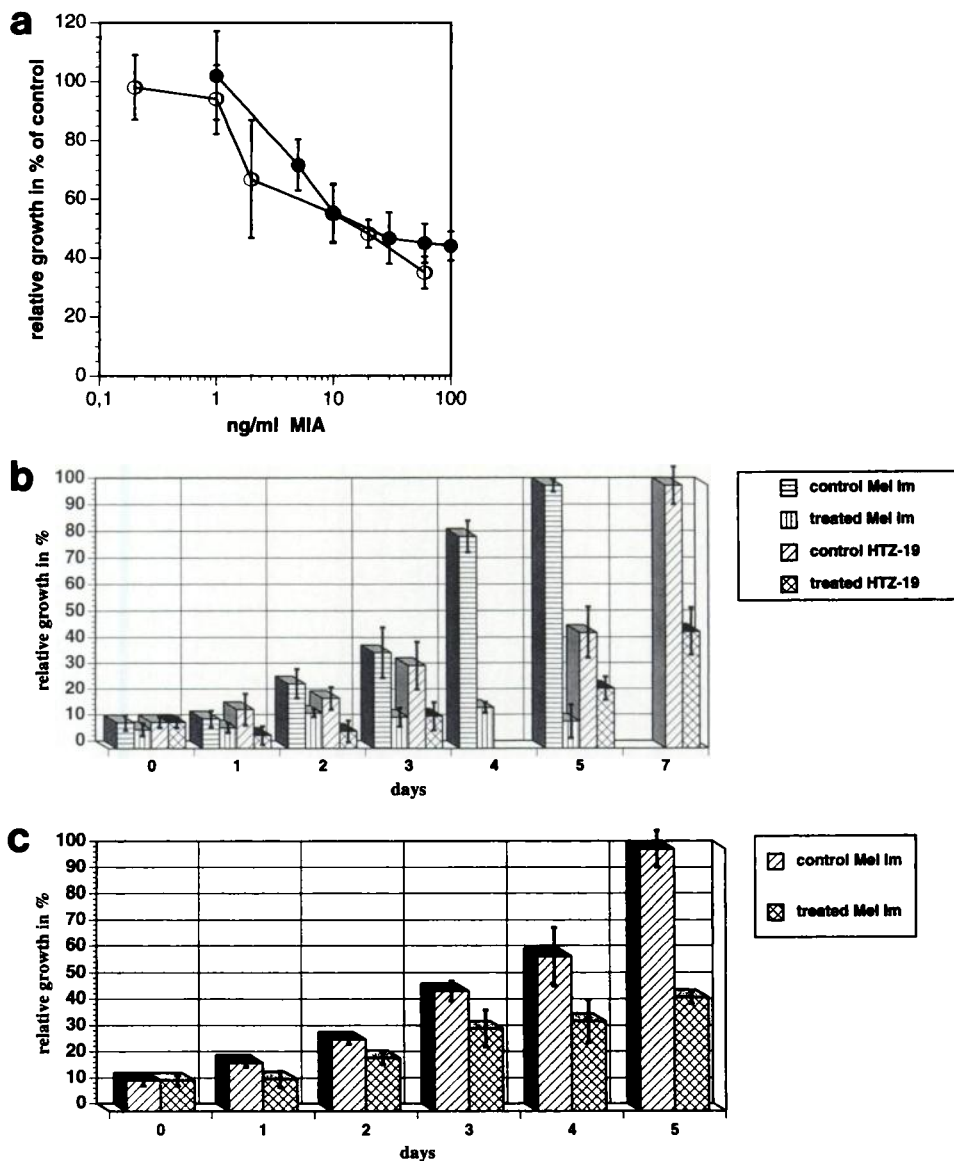
Fig. 5. Biological activity of recombinant MIA protein. A , dose-response curves of the melanoma cell lines HTZ-19 (●) and Mel Im (○). Cells were treated for 5 days with the indicated doses of prokaryotic expressed MIA; relative growth was determined by counting cells treated with recombinant MIA compared to controls treated with identically purified protein from E. coli bearing the empty vector pQE-40. Protein concentrations were estimated by comparing the intensity of silver staining of MIA with standard proteins in SDS-gels. B , cell growth curves of HTZ-19 and Mel Im after treatment with recombinant huMIA, expressed in E. coli . Controls were treated with identically purified protein from E. coli bearing the empty vector pQE-40 (relative growth is given in a percentage \pm SD). C , cell growth curve of Mel Im after treatment with supernatants containing eukaryotic expressed recombinant huMIA. Controls were treated with supernatants of the PA-1 cells transfected with the empty vector (relative growth is given in percentage \pm SD).
