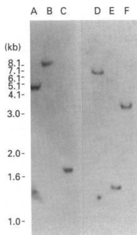
Fig. 5. Southern blot analysis of human genomic DNA
