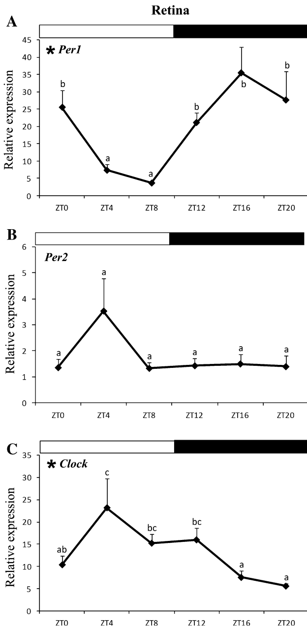
Fig. 3 Relative expression of Per1 (a), Per2 (b), and Clock (c) in Senegalese sole retina during the daily light–dark (LD) cycle. Samples were taken every 4 h and each value represents the mean ± SEM of six different specimens ( n = 6 ). The bars above each graph indicate the daily photoperiod conditions. White bars represent the daily light phase (sampling points ZT0, ZT4 and ZT8) and black bars represent phases of darkness (sampling points ZT12, ZT16 and ZT20). Different letters indicate statistically significant differences between mean values ( p < 0.05 ). The asterisk indicates a significant rhythm by cosinor analysis (see Table 2 for details)
