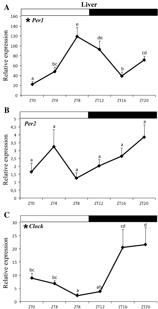
Fig. 7 Relative expression of Per1 (a), Per2 (b), and Clock (c) in the liver of Senegalese sole during the daily LD cycle. For further details, see the legend of Fig. 3
