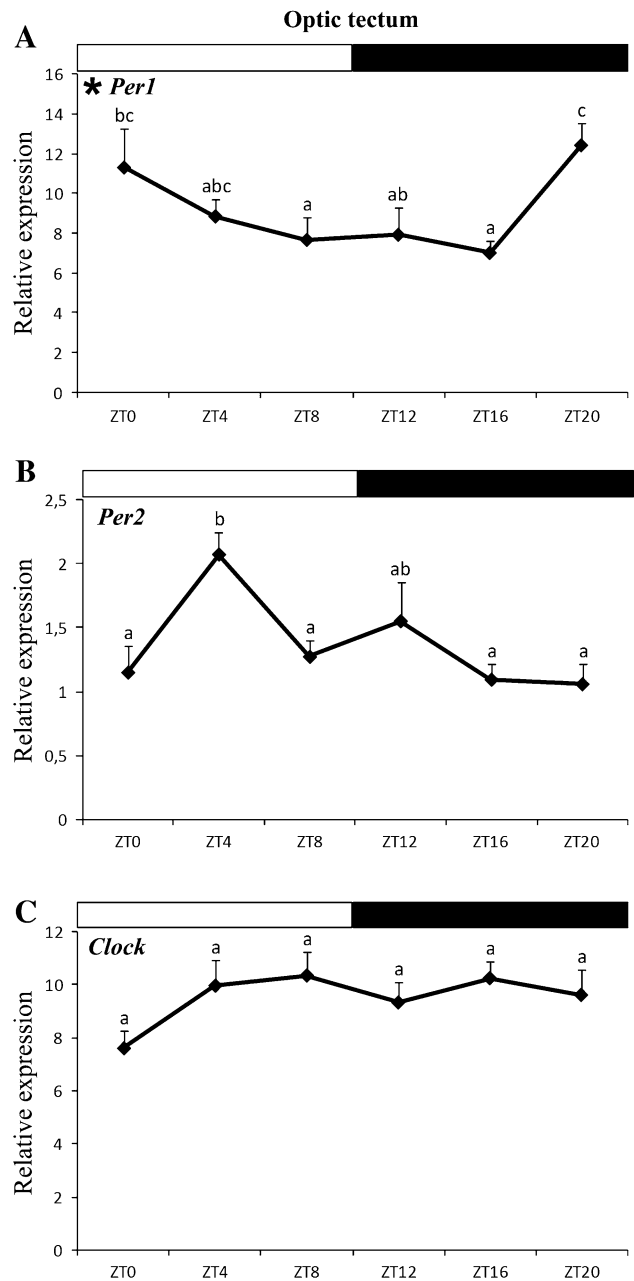
Fig. 4 Relative expression of Per1 (a), Per2 (b), and Clock (c) in Senegalese sole optic tectum during the daily LD cycle. For further details, see the legend of Fig. 3
