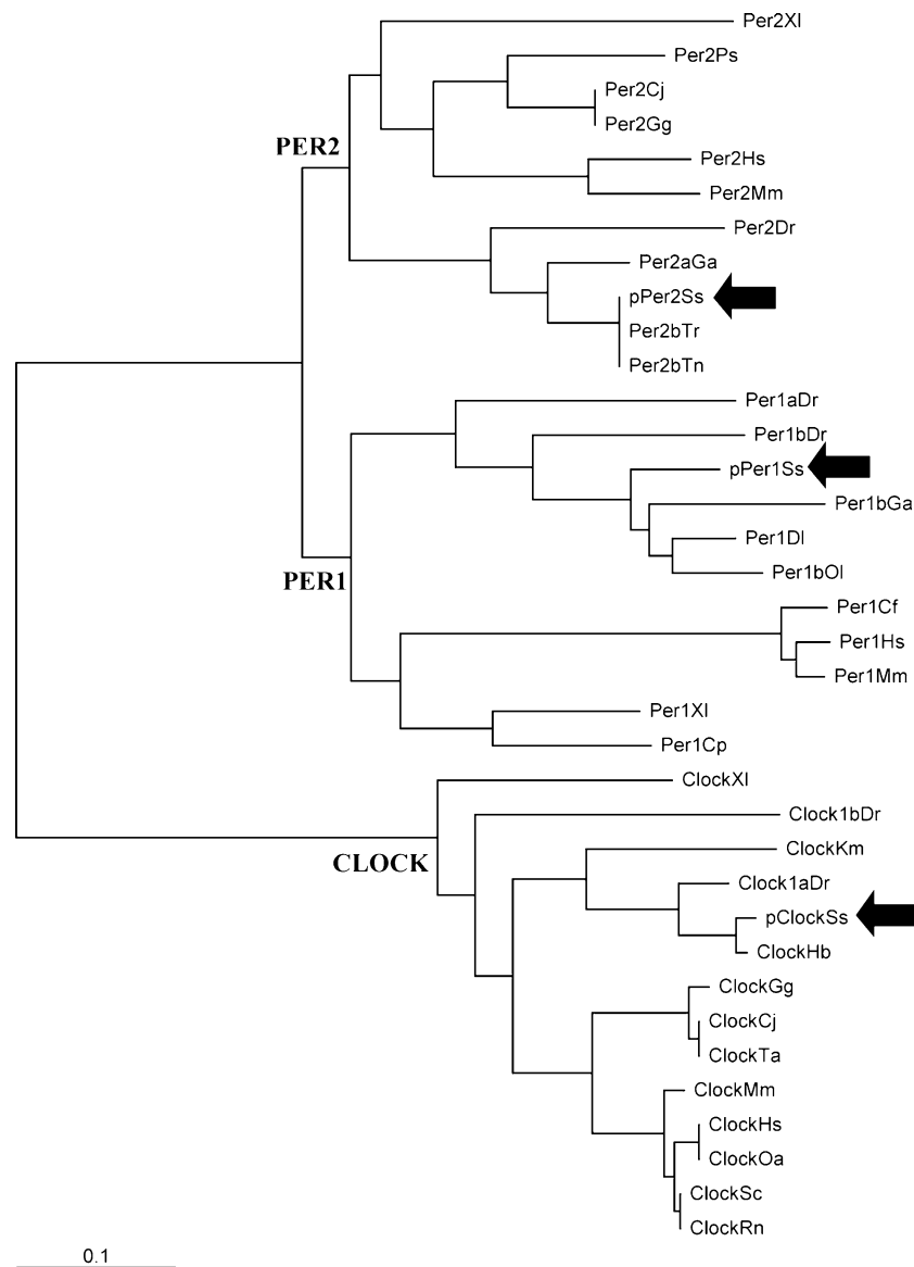
Fig. 1 Phylogenetic tree of PER and CLOCK proteins created by the neighbor-joining method. Only complete protein sequences were used for the analysis. The length of the branches is proportional to the phylogenetic distance. Solea senegalensis circadian proteins positions are indicated by black arrows. Cf, Canis familiaris ; Cj, Coturnix japonica ; Cp, Cynops pyrrhogaster ; Dl, Dicentrarchus labrax ; Dr, Danio rerio ; Ga, Gasterosteus aculeatus ; Gg, Gallus gallus ; Hb, Haplochromis burtoni ; Hs, Homo sapiens ; Km, Kryptolebias marmoratus ; Mm, Mus musculus ; Oa, Ovis aries ; Ol, Oryzias latipes ; Ps, Podarcis sicula ; Sc, Spalax carmeli ; Rn, Rattus norvegicus ; Ss, Solea senegalensis ; Ta, Tyto alba ; Tn, Tetraodon nigroviridis ; Tr, Takifugu rubripes ; XI, Xenopus laevis . Protein accession numbers and Ensembl protein IDs used for alignment and phylogenetic analysis were the following: ENSCAF00000025009 ( Canis familiaris PER1); BAB03455, BAB03454, ( Coturnix japonica PER2, CLOCK); BAC98490 ( Cynops pyrrhogaster PER1); GQ353293 ( Dicentrarchus labrax PER1); NP_001025354, NP_997604, NP_878277, NP_571032, NP_840080
