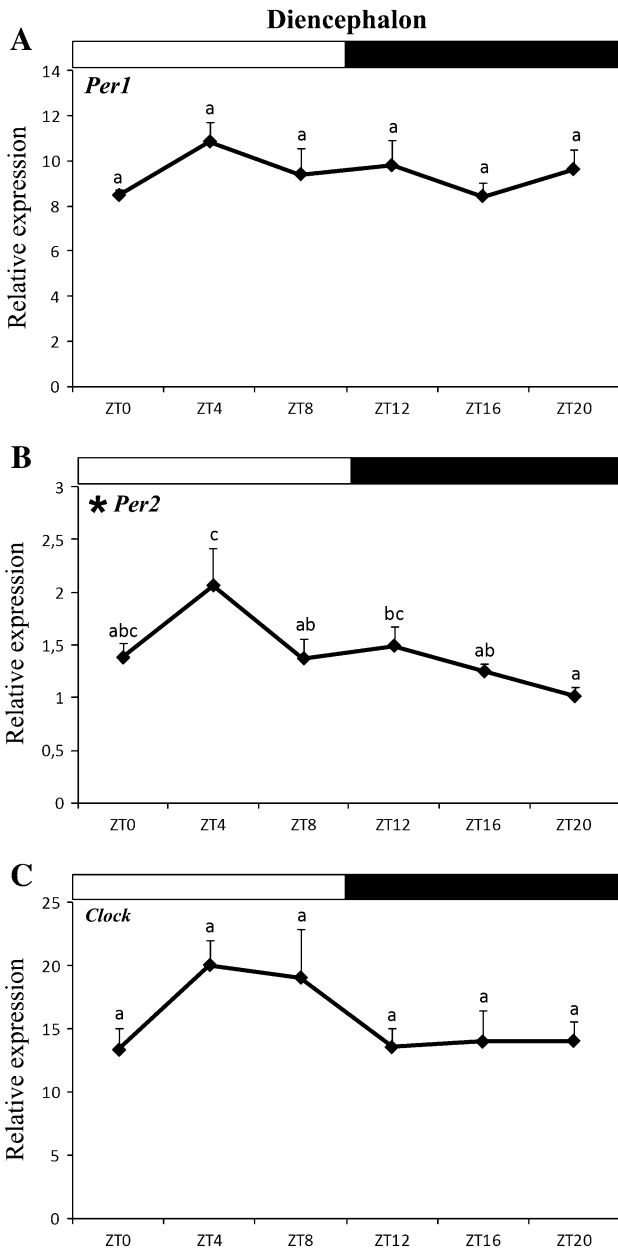
Fig. 5 Relative expression of Per1 (a), Per2 (b), and Clock (c) in the diencephalon of Senegalese sole during the daily LD cycle. For further details, see the legend of Fig. 3
