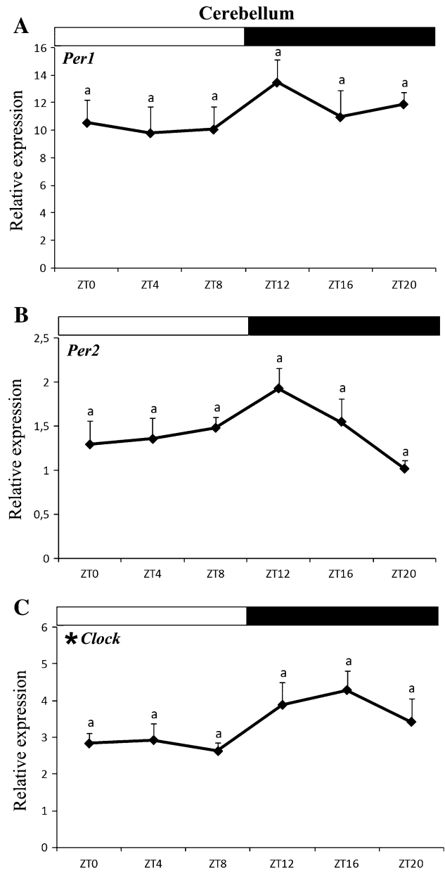
Fig. 6 Relative expression of Per1 (a), Per2 (b), and Clock (c) in the cerebellum of Senegalese sole during the daily LD cycle. For further details, see the legend of Fig. 3
