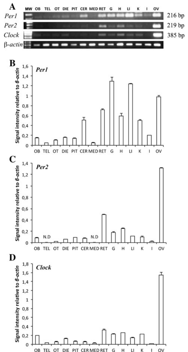
Fig. 2 Tissue distribution of Senegalese sole clock genes in central and peripheral tissues. a Specific Per1 , Per2 , and Clock products of 216, 219, and 385 bp, respectively, were amplified following the RT-PCR conditions described in “Materials and methods”. Sole \beta -actin was used as internal control gene (lower panel). b–d Signal intensity of above amplified products relative to \beta -actin for Per1 ( b ), Per2 ( c ), and Clock ( d ) was calculated by using the Quantity one ® software (Bio-Rad). Columns represent the mean \pm SEM of three different measurements. Per2 signal was not detected in telencephalon and medulla. MW molecular weight marker (100-bp Dominion, Córdoba, Spain), OB olfactory bulbs, TEL telencephalon, OT optic tectum, DIE diencephalon, PIT pituitary, CER cerebellum, MED medulla, RET retina, G gills, H heart, LI liver, K kidney, I intestine, OV ovary, N.D. non-detected
