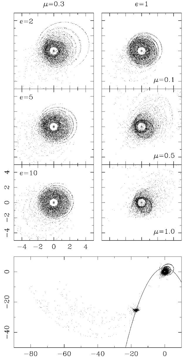
Figure 18. Summary of coplanar model results in face-on particle plots. The models were run for 120 time units, with the perturber initialized a radial distance of 20 units from the primary. After much longer times the phase mixing in the particles' orbits results in dissolution of the ring features, maintaining the distended envelopes of the discs seen above. The position of the primary is plotted with an asterisk. The top left-hand side panel shows results for models with \mu = 0.3 and from top to bottom e = 2, 5 and 10 respectively. The top right-hand side panel shows results for models with e = 1 and from top to bottom \mu = 0.1, 0.5 and 1 respectively. The bottom panel shows results, on a larger scale, for the model with e = 1 and \mu = 0.3 . The perturber trajectory is shown with a solid line. We see: the perturbed disc with rings, the captured particles clustered about the instantaneous position of the perturber, and escaping particles (the large arcs on the left-hand side of the plot).
