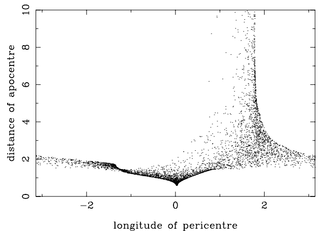
Figure 8. The final distance of apocentre against the longitude of pericentre for a fly-by simulation with a parabolic perturber orbit in which only the direct tidal potential has been used. Data correspond to those given in Fig. 4.
