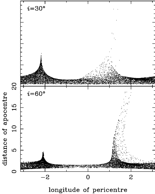
Figure 11. The final distance of apocentre against the longitude of pericentre for parabolic fly-by simulations with orbital inclination i = 30^\circ and 60^\circ .
