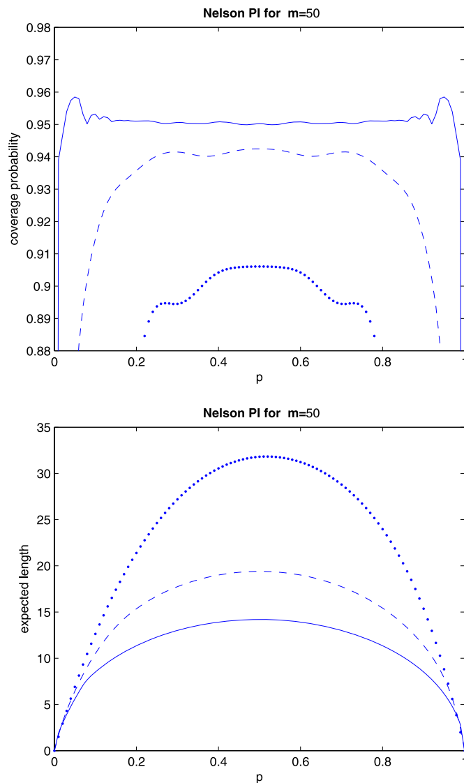
Figure 1. Coverage probabilities and expected lengths of the 95% level Nelson prediction intervals for the Binomial distributions with n = 10 (dotted line), n = 50 (dashed line), and n = 1000 (solid line). The online version of this figure is in color.
