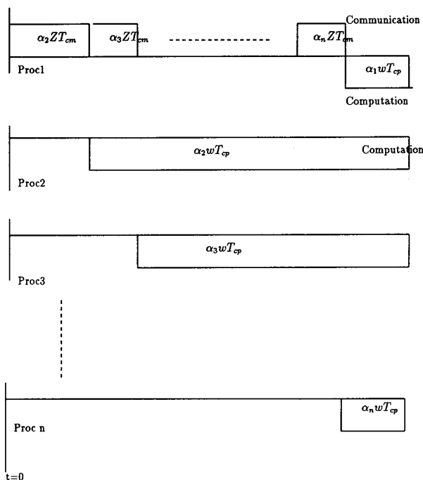
Fig. 3. Timing diagram for homogeneous bus network without front-end processors.
