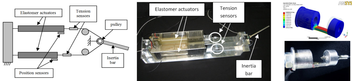
Figure 1: sketch (a), and picture of the experimental setup (b). Two dielectric elastomer actuators arranged in antagonistic configuration are employed to move a pulley, on which a link is attached. Position sensors and tension sensors are employed to measure the displacement and the forces developed by the actuators (c).
