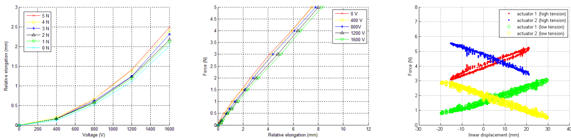
Figure 2: Voltage-elongation (a) and force-elongation (b) relationship of one of the two elastomer actuators, expressed as a function of an externally applied load and an externally applied voltage respectively.
