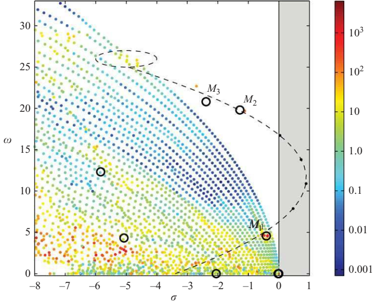
FIGURE 10. Eigenvalues of the reduced matrix \hat{\mathbf{A}}_{\hat{p}, \hat{p}} superimposed on the global spectrum of the cavity. Eight unstable global modes and 13 BPOD modes have been included in the reduced model. The global spectrum is coloured according to the criterion \Gamma_i .
