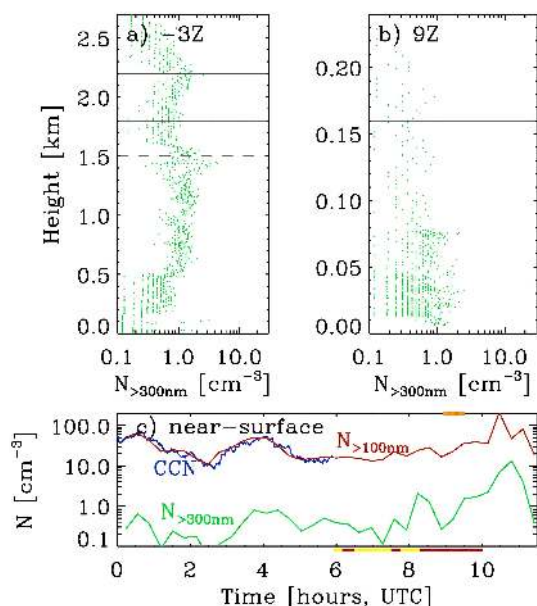
Fig. 11. Near-surface and helicopter aerosol measurements on 25 August 2008 (Case #3), including helicopter profiles of aerosol concentration for particles larger than 300 nm taken (a) about 3 h prior to 0Z and (b) 9Z, and (c) concentrations of CCN (blue), aerosols larger than 100 nm (red) and aerosols larger than 300 nm (green) measured onboard Oden . In (a–b), the solid and dashed lines are the cloud boundaries and mixed-layer base heights determined by remote sensors at the time, respectively. Red bars on the lower axis of (c) indicate questionable data due to contamination (yellow bars may also be questionable due to temporal proximity), while the orange bar on the top axis shows the time of the second helicopter profile. Note the different vertical scales for (a) and (b).
