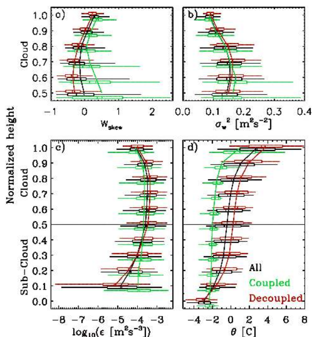
Fig. 14. Normalized statistical profiles of (a) vertical velocity skewness, (b) vertical velocity variance, (c) turbulent dissipation rate, and (d) 60-GHz radiometer-derived potential temperature. Black curves represent all data noted by the thick black lines at the top of Fig. 12, while the red and green curves are for the predominantly decoupled and intermittently coupled time periods noted in Fig. 12, respectively. Normalization is done relative to the cloud top (1.0), cloud base (0.5), and surface (0.0) in steps of 0.1. At each normalized height level, box-and-whisker diagrams show the 5th, 25th, 50th, 75th, and 95th percentiles, while the continuous vertical curves represent the mean values. Statistics are computed at the same normalized heights for all data subsets, but are visualized at slightly different heights to facilitate comparisons. Since vertical velocity can only be determined within cloud layers, (a) and (b) only show normalized height ranges within cloud.
