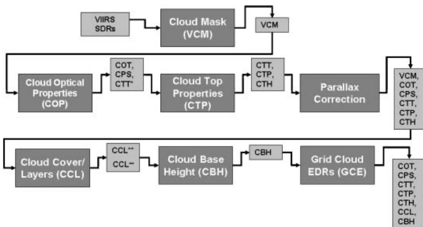
Figure 1. Architecture of the VIIRS cloud algorithms. COT, cloud optical thickness; CPS, cloud effective particle size; CTH, cloud top height; CTT, cloud top temperature; SDR, VIIRS sensor data records; VCM, VIIRS cloud mask
