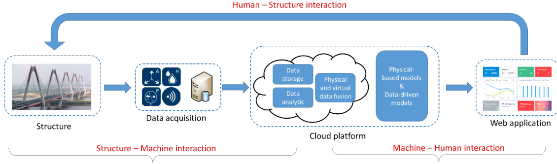
Fig. 2. A Cloud based Digital Twin model
