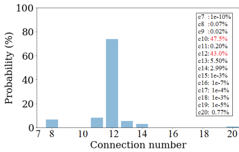
Fig. 11. Predicted probability for all classes at IDCNN's output layer.
