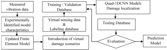
Fig. 9. Workflow of training process for CNN-based SHM.
