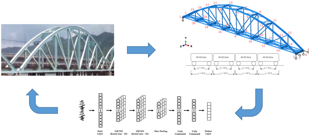
Fig. 8. Architecture of the Deep CNN algorithm designed for structural damage detection.
