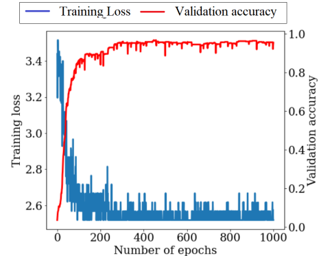
Fig. 10. Evolution of train and validation loss during the training process.
