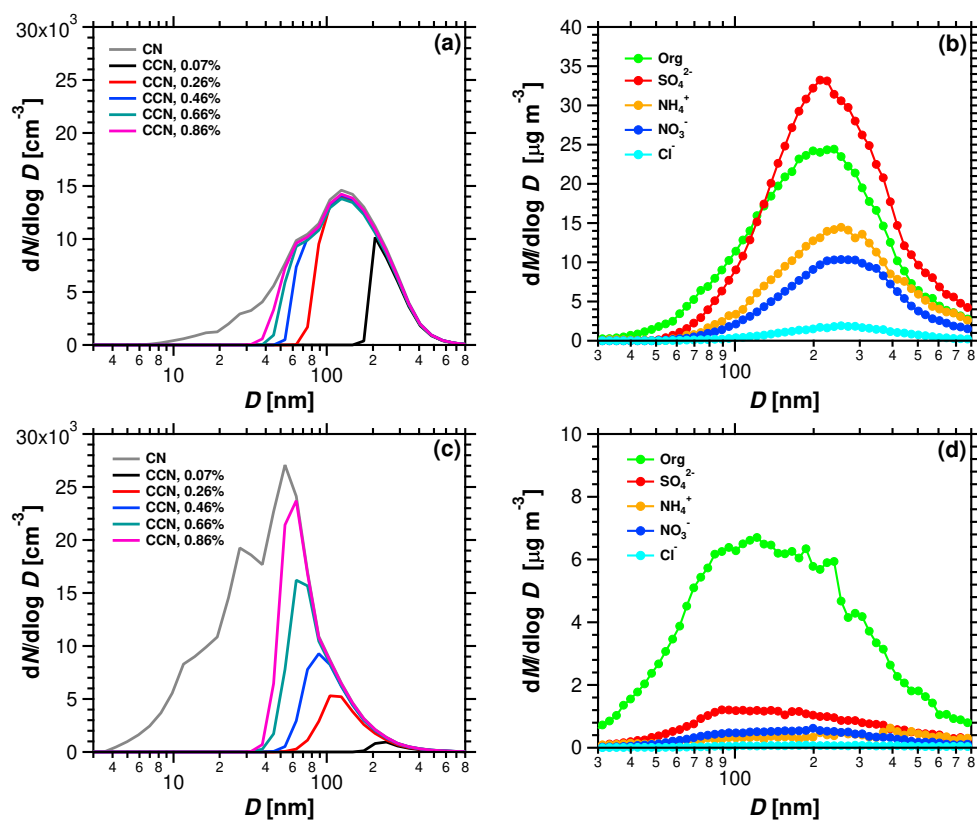
Fig. 4. Number size distributions of total aerosol particles (CN) and of cloud condensation nuclei (CCN) for different supersaturation levels (left column; panels a , c ), and mass size distributions of organic and inorganic compounds determined by AMS (right column; panels b , d ). The upper panels ( a , b ) are averages over the aged regional pollution period and the lower panels ( c , d ) are averages over the fresh city pollution period.
