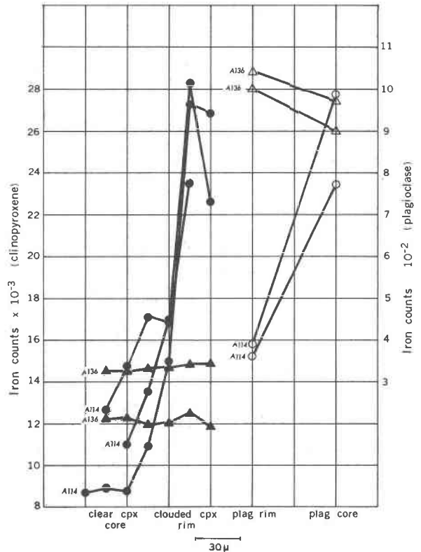
FIG. 5. X-ray intensity (counting interval about 20 seconds, terminated on fixed beam current) of iron in clinopyroxene (solid) and plagioclase (open) in metadolerite (circles) and quartz dolerite (triangles).
