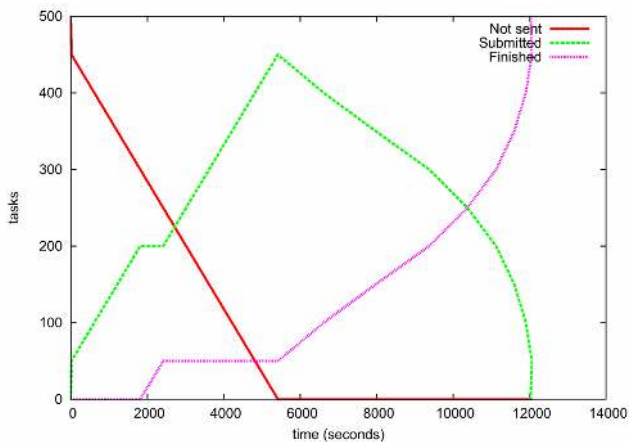
Figure 9. Task execution with time-shared scheduling of tasks.
