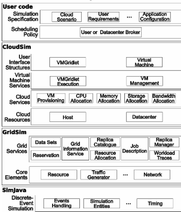
Figure 2. Layered CloudSim architecture.
