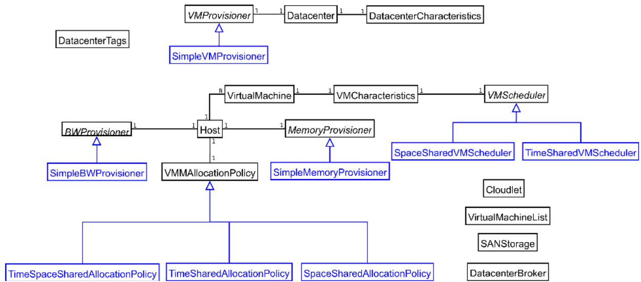
Figure 4. CloudSim class design diagram.
