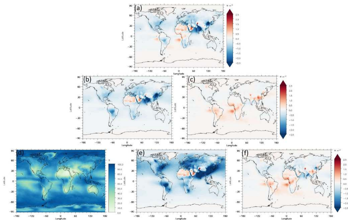
Figure 2. Annual-mean all-sky anthropogenic \text{RF}_{\text{ari}} and various terms from clear and cloudy skies simulated with OsloCTM3 (Lund et al., 2018). The panel in the top row shows the all-sky \text{RF}_{\text{ari}} (a); the second row shows the contributions from clear ( \text{RF}_{\text{ari,clear}} ) and cloudy skies ( \text{RF}_{\text{ari,cloud}} ) (first, b, and second term, c, on the right-hand side on Eq. 1, respectively). The third row shows cloud fraction (AC) (d), \text{RF}_{\text{ari,total-clear}} (e) and \text{RF}_{\text{ari,total-cloud}} (f), respectively. Panel (d) on cloud fraction is shown in percent, and the other panels are in watts per square metre.
