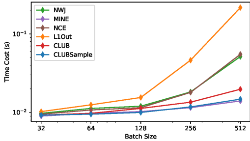
Figure 3. Estimator speed comparison with different batch size. Both the axes have a logarithm scale.
