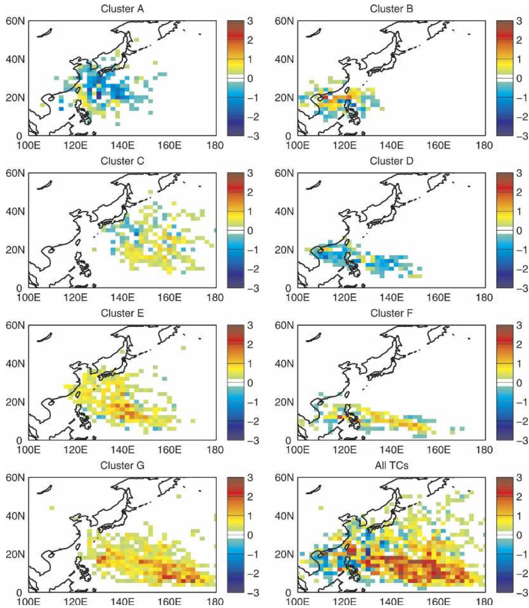
FIG. 14. Track density difference between El Niño and La Niña years for each cluster and all TCs; the resolution is 2^\circ \times 2^\circ .
