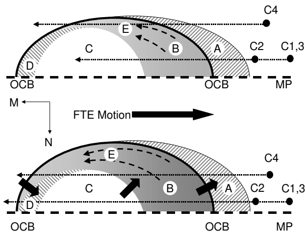
Fig. 9. A possible interpretation of the PEACE observations for the internal structure of FTEs. In each panel, the FTE is assumed to be a bundle of reconnected flux tubes occupying the region between the unperturbed magnetopause (dashed horizontal line marked MP) and an internal boundary between the open and closed flux tubes (represented by the curved solid line marked OCB at each end). The relative trajectories of the 4 spacecraft are represented by the horizontal dotted arrowed lines, which point left as the FTE motion is in the negative M direction, i.e. to the right. The observation of enhanced field strengths and densities of magnetospheric electrons prior to the arrival of the magnetosheath electrons implies a compressed region (marked A) on the closed flux tubes ahead of the FTE. On crossing the OCB, the spacecraft will observe a sudden enhancement of magnetosheath electrons on the oldest reconnected field lines (marked B). On moving further into the FTE, the spacecraft move onto more recently reconnected field lines, which may not yet have completely filled with magnetosheath plasma, and thus observe a declining density (marked C). It appears that an enhancement in magnetospheric electrons occurs in the trailing edge of the FTE (marked D). In order to explain the delayed and extended signature at C4, it is necessary to account for magnetosheath electrons in the region marked E in the figures. We infer a re-circulation of the oldest reconnected flux tubes along the leading edge of the FTE structure, as indicated by the dashed arrowed lines. During the first event, represented by the upper figure, we suggest that C4 passes through this region, then out across the OCB and back onto closed field lines and thus does not observe the magnetospheric population marked D. During the second event studied in this paper, represented in the lower figure, we infer that C4 passed relatively deeper into the FTE, and that the re-circulation of the oldest flux tubes had proceeded sufficiently to push some of these flux tubes as far back as the trailing edge of the FTE. Therefore, all 4 spacecraft observe a second enhancement of magnetosheath electrons after the magnetospheric population (D). In addition, this interpretation is consistent with the inferred motion of the 4 boundaries shown in Fig. 8, as indicated by the heavy arrows in the lower figure.
