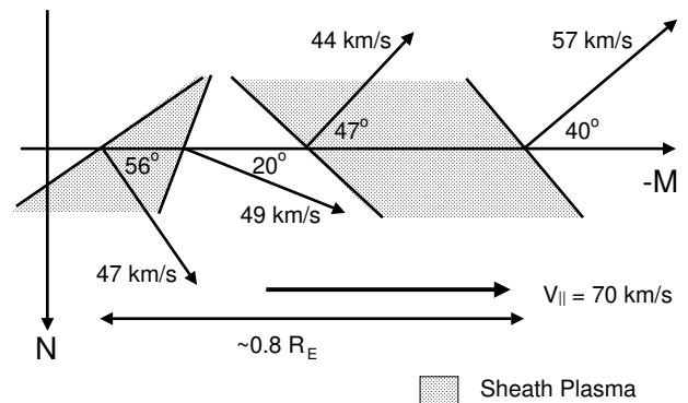
Fig. 8. A summary sketch of the inferred orientation and motion of the observed boundaries of magnetosheath electron populations shown in Fig. 7. The leading edge of the first, major enhancement, represented on right, moves duskward and Earthward at 57 \text{ km s}^{-1} . Somewhat unexpectedly, the trailing edge of this enhancement (second from right) has a similar motion. However, the leading and trailing edges of the more minor enhancement in magnetosheath density show motion towards dusk and back out towards the magnetopause. Note that the positions of the boundaries on the M axis are scaled according to the times of their observation, in order to represent an approximate spatial separation of these structures. The inferred motion is consistent with the entire structure having a scale size of \sim 0.8 R_E and moving duskwards across the magnetopause at \sim 70 \text{ km s}^{-1} .
