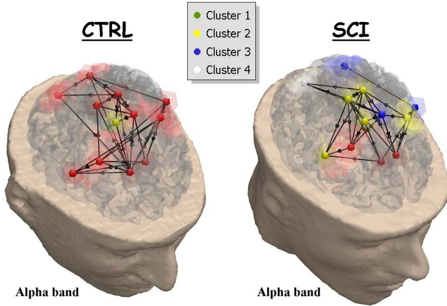
Fig. 4. Graphical representation of the identified clusters of ROIs within the functional networks estimated from a representative control (CTRL) subject and spinal cord injured (SCI) patient during the movement preparation in the Alpha band. The functional network is illustrated as a three-dimensional graph on the realistic cortex model. Spheres located at the barycenter of each ROI represent nodes. Black directed arrows represent edges. The graph partitioning is illustrated through the nodes coloring. Nodes with same colors belong to the same cluster.
