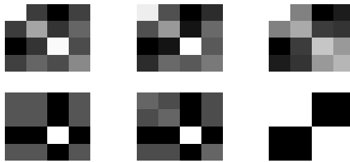
Figure 2: Recovered \Sigma with CN (upper line) and k -means (lower line) for 28, 50 and 100 points.
