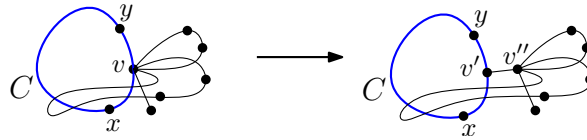
Figure 9: Splitting a vertex v common to several cycles in G'[A] .
