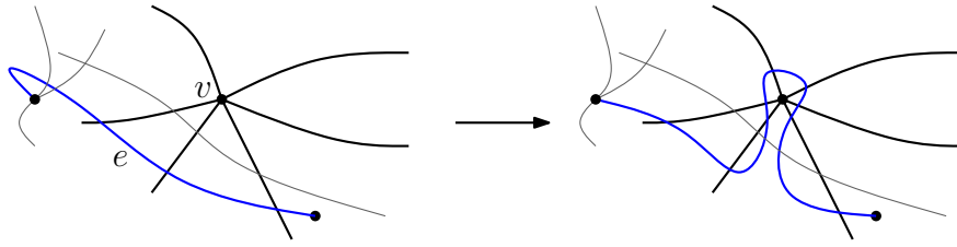
Figure 3: A continuous deformation of e resulting in an edge-vertex switch (e, v) .
