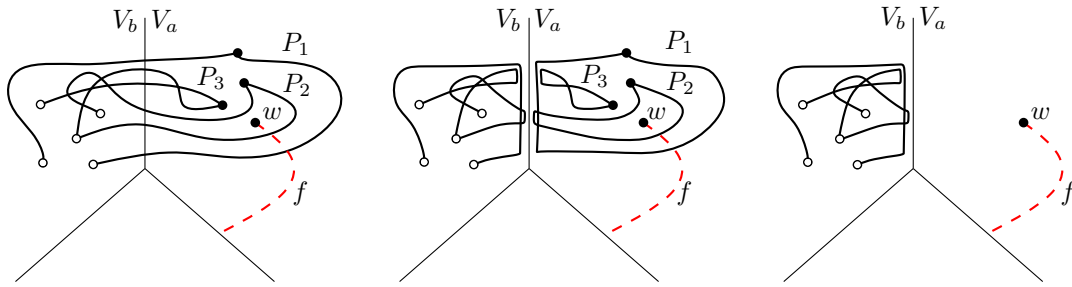
Figure 14: Illustration for the proof of Lemma 12. From left to right: the successive stages of the redrawing operation eliminating paths P_1, P_2 and P_3 . The edge f cannot be present in the drawing, since it would violate its evenness.
