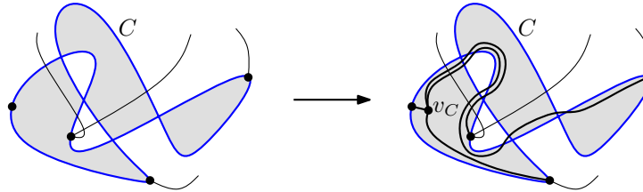
Figure 9: Splitting a vertex v common to several cycles in G'[A] .
