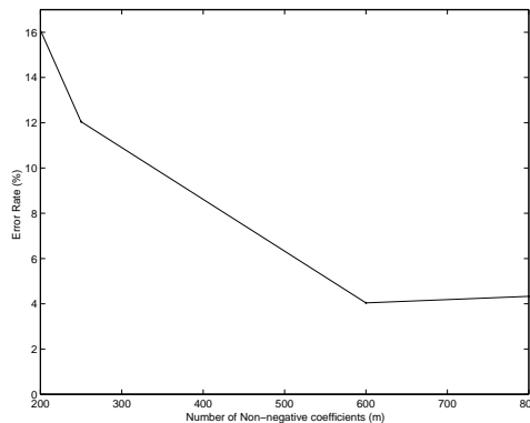
Figure 8: Effects of parameter selection on clustering results with the PIE 66 (frontal) database.
