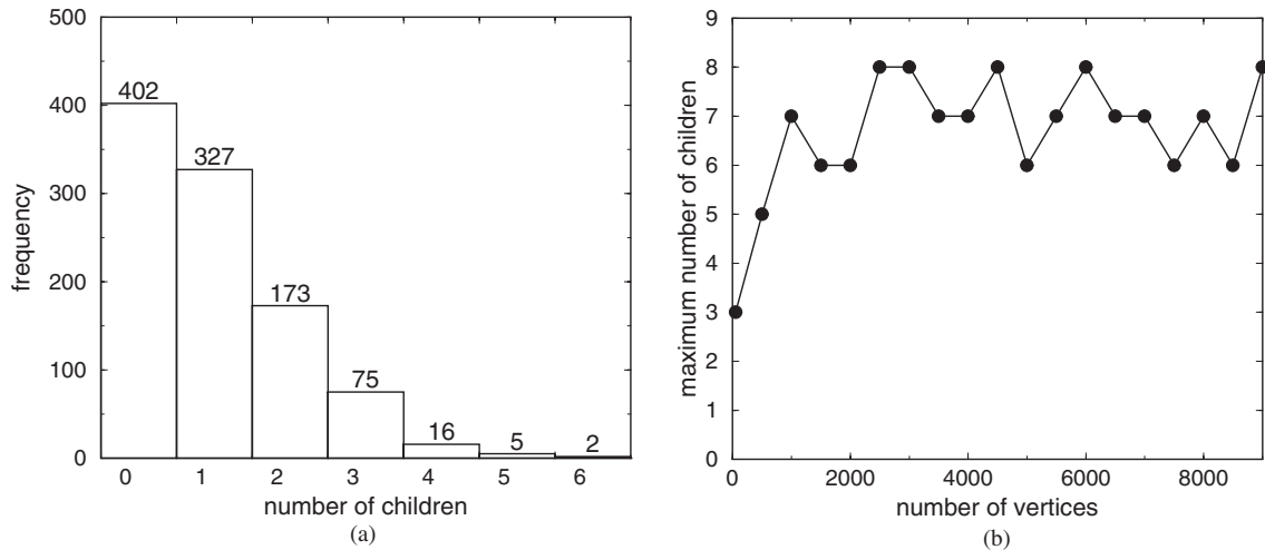
Fig. 5. (a) The distribution of the number of children of the MST representing a data set with 1000 random data points in 60-dimensional Euclidean space. (b) The maximum number of children versus the total number of data points ranging from 50 to 9000.
