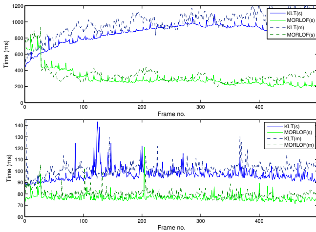
Figure 7. Top: (a) Execution time for the static sequence (s) and the hand-held captured sequence (m) with CPU implementations. Bottom: (b) Execution time with the GPU implementations.
