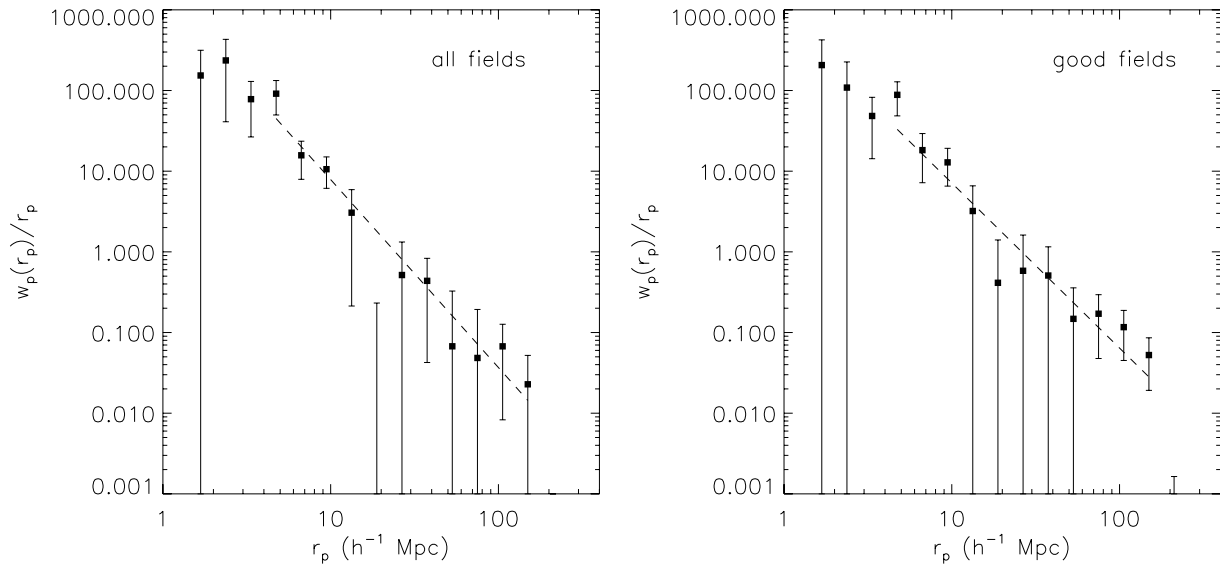
FIG. 5.— Projected correlation function w_p(r_p) for the z \geq 2.9 quasars. Errors are estimated using the jackknife method. Also plotted are the best fitted power-law functions, with fitted parameters listed in Table 4. left : for all fields; right : for good fields only. The two cases give similar results.
