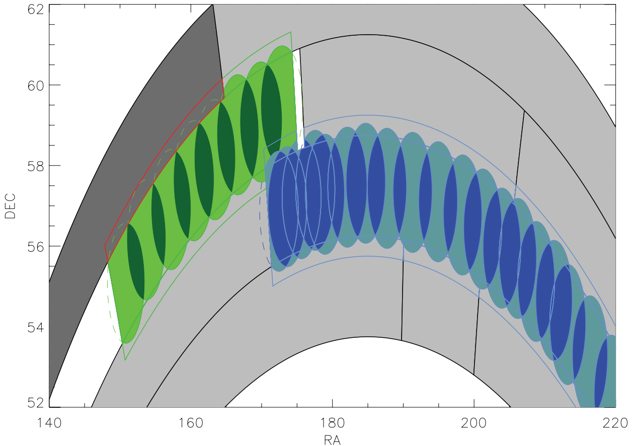
FIG. B1.— Portion of the targeting and tiling geometry in SDSS spectroscopy. The targeting chunks are denoted by stripes bounded by black lines and each targeting chunk is targeted using one target version. Gray stripes are targeting chunks with target version no lower than v3.1.0 (not necessarily the same version); one dark gray targeting chunk shown here is targeted with target version v2.13.5 . Within targeting chunks we carve out tiling rectangles, each of which is targeted with a unique version. A set of tiling rectangles form a tiling chunk. Shown here as examples are tiling chunk 38, which has one rectangle (red) targeted with version v2.13.5 and three rectangles (green) with version v3.1.0 ; tiling chunk 67, whose rectangles (blue) are all with target version v3.1.0 or later. Within each tiling chunk we place tiles ( 1^\circ.49 radius circles, which appear as ellipses because the aspect ratio of the region of sky shown is not 1 : 1 ); tiles are trimmed by the boundaries of rectangles of that tiling chunk and balkanized (i.e., Hamilton & Tegmark 2004) into non-overlap sectors (which are covered by only one tile) and overlap sectors (which are covered by more than one tile). We use light and dark colors to denote the two types of sectors in the above two tiling chunks. Note that though balkanized sectors of the same tiling chunk do not intersect with each other, they could intersect with sectors of another tiling chunk. In the above case, the upper-left corner rectangle in tiling chunk 67 is completely within the middle main rectangle of tiling chunk 38. Therefore one should be careful when computing the effective area of sectors. In constructing our clean subsample for clustering analysis, we reject those sectors that are within tiling rectangles which are targeted with target version lower than v3.1.0 , i.e., regions such as the red rectangle in chunk 38.
