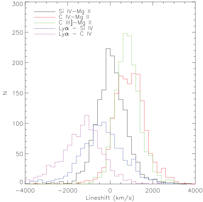
FIG. A1.— Distributions of relative shifts of the modes of various emission lines, as measured for 1652 high S/N, non-BAL quasars with redshifts between 1.8 and 2.2. The mean values and 1-\sigma deviations of these line shifts are listed in Table A1.
