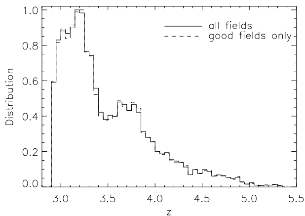
FIG. 2.— Observed redshift distribution of our quasar clustering subsamples, normalized by the peak value. This distribution is the product of the evolution of the quasar density distribution, and the quasar selection function; the latter is responsible for the dip at z \approx 3.5 , where quasars have very similar colors to those of G and K stars. We show the redshift distributions for the subsamples both including and excluding bad fields; the results are essentially identical. The redshift binning is \Delta z = 0.05 .
