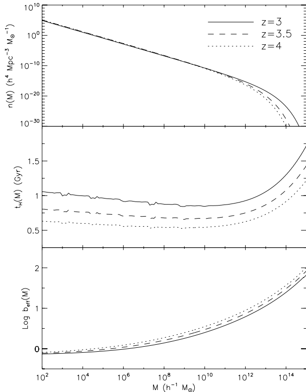
FIG. 8.— The Sheth & Tormen (1999) halo mass function, halo lifetime and effective bias factors for halos with M > M_{\text{min}} as functions of halo mass for three redshifts z = 3, 3.5, 4 , in our fiducial cosmology. The age of the universe at these three redshifts is 2.2, 1.9, and 1.6 Gyr, respectively, and for typical halos with a mass of a few \times 10^{12} h^{-1} M_{\odot} , the halo lifetime is approximately 0.7 \sim 1 Gyr at these redshifts.
