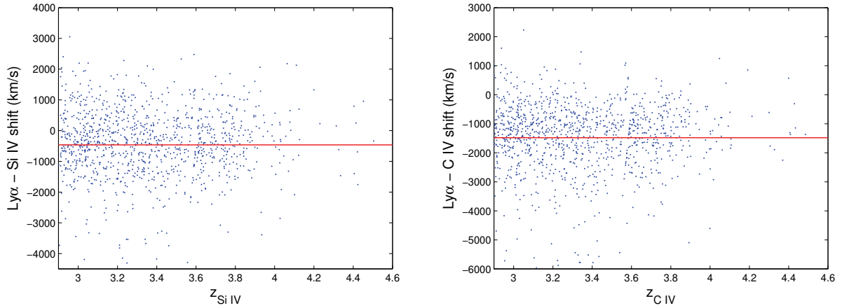
FIG. A3.— Relative shifts of \text{Ly } \alpha versus \text{SiIV} and \text{CIV} emission lines as a function of redshift. Red lines indicate the mean value of line shifts. The mean values of line shifts and 1-\sigma deviations are listed in Table A1.
