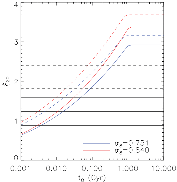
FIG. 10.— Comparison of the measured and model predicted clustering strength \xi_{20} , defined in equation (7). Solid lines correspond to the 2.9 \leq z \leq 3.5 bin and dashed lines correspond to the z \geq 3.5 bin. The thick and light horizontal lines show the measured clustering strength and 1 - \sigma errors. The match of the model predicted \xi_{20} (blue lines for the fiducial \sigma_8 = 0.751 and red lines for \sigma_8 = 0.84 ) with the measured \xi_{20} gives the average quasar lifetime t_Q within that redshift bin. The uncertainty in measured \xi_{20} gives a large uncertainty in t_Q . Quasars in the higher redshift bin have larger t_Q on average. The fiducial values of t_Q inferred from this figure (the \sigma_8 = 0.751 case) are: t_Q = 15 Myr for 2.9 \leq z \leq 3.5 and t_Q = 160 Myr for z \geq 3.5 .
