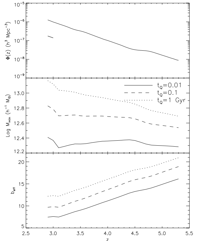
FIG. 9.— The top panel shows the integrated quasar luminosity function (LF) down to the magnitude cut i = 20.2 , computed using the variable power-law fit function in Richards et al. (2006). The lower line segment shows the integrated LF down to i = 19.1 . The bottom two panels show the computed minimum halo masses and effective bias factors as functions of redshift, for the three trial values of t_Q = 0.01, 0.1 and 1 Gyr. We have used the empirical values of \Phi at the grid points z = 2.9, \text{ and } 3.0 (i.e., three and four times the values down to i = 19.1 , respectively), which causes the jump in M_{\text{min}} and b_{\text{eff}} at these two redshift grid points, i.e., we are targeting more luminous quasars at z = 2.9, 3.0 . The slight kink around z = 4.5 in all three panels is due to the K-correction (see figure 17 of Richards et al. 2006).
