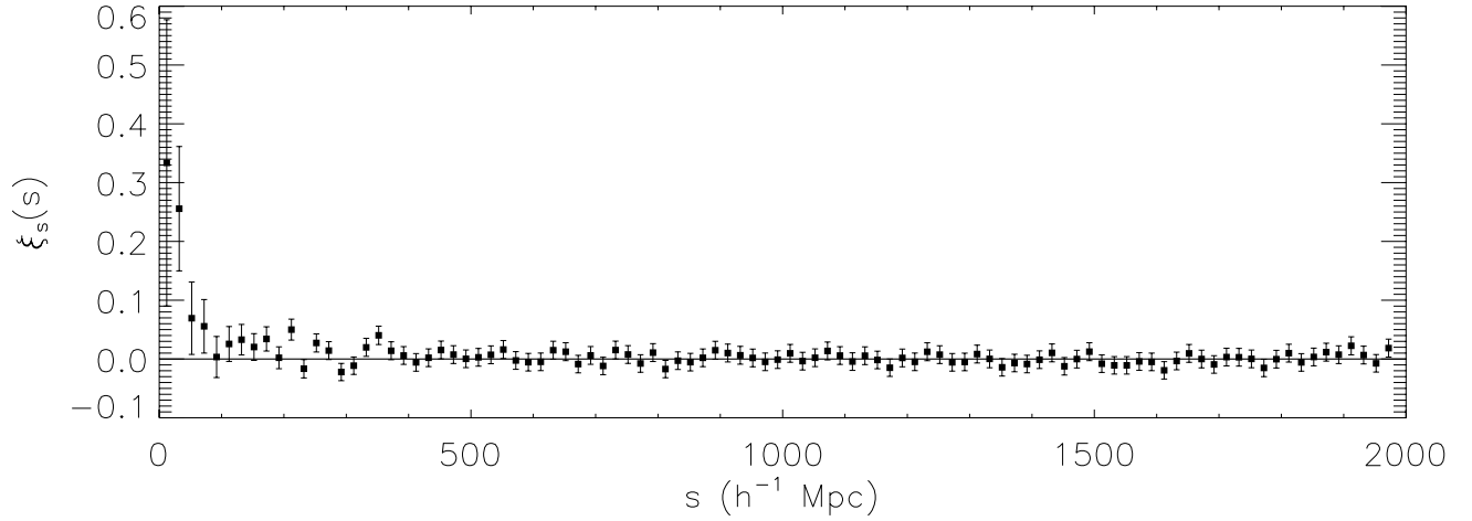
FIG. 4.— Large scale behavior of \xi_s(s) for the z \geq 2.9 quasars (all fields included). Errors are estimated using the Poisson estimator. The redshift space correlation function essentially vanishes after s > 200 h^{-1} Mpc, with a mean of 0.002 and rms scatter \pm 0.01 in the range 200 < s < 2000 h^{-1} Mpc.
