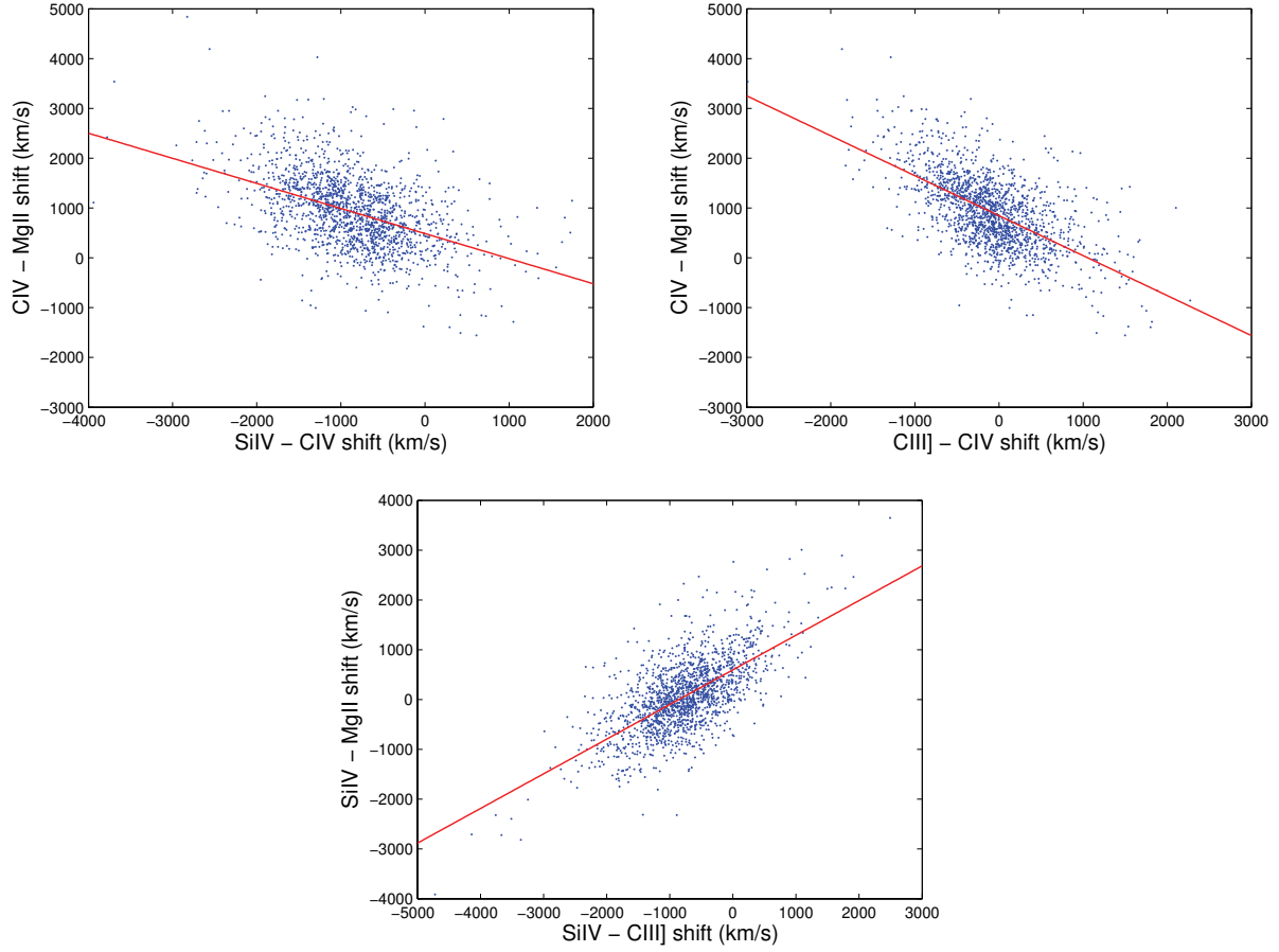
FIG. A2.— Correlations between various emission line shifts. Blue dots are data points and red lines are fitted linear functions. These correlations are used in our redshift estimation. The fitted linear parameters and 1-\sigma deviations are listed in Table A1.
